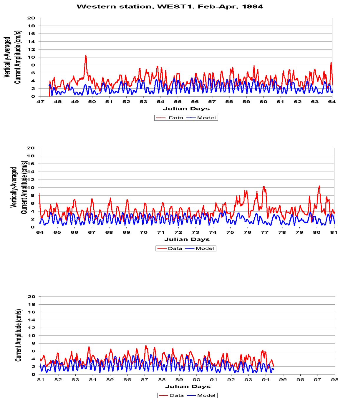
Figure 11a. Comparison of predicted and measured current amplitudes at WEST1
