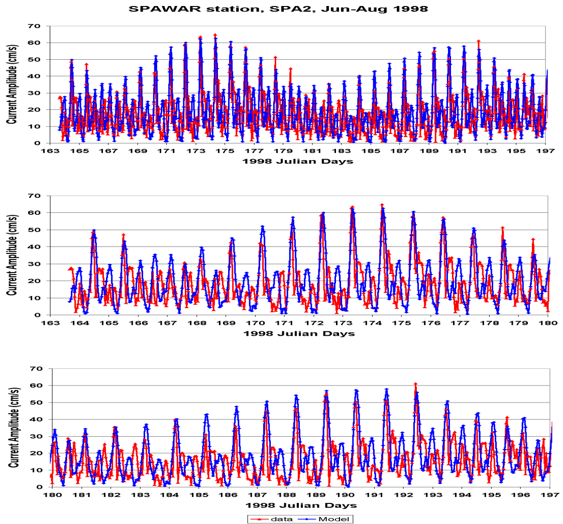
Figure 16a. Comparisons of predicted and measured current amplitudes at SPA2
