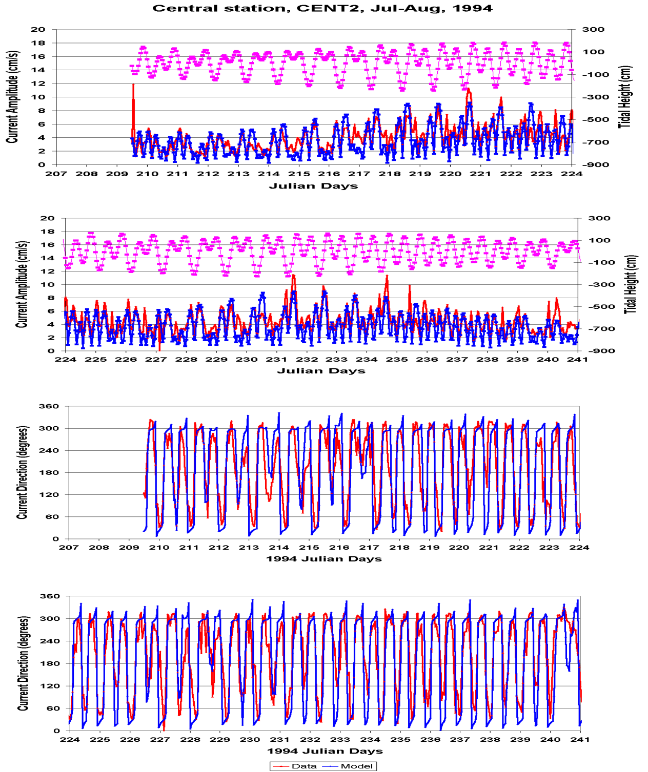
Figure 12. Comparisons of predicted and measured current amplitudes and directions at CENT2
