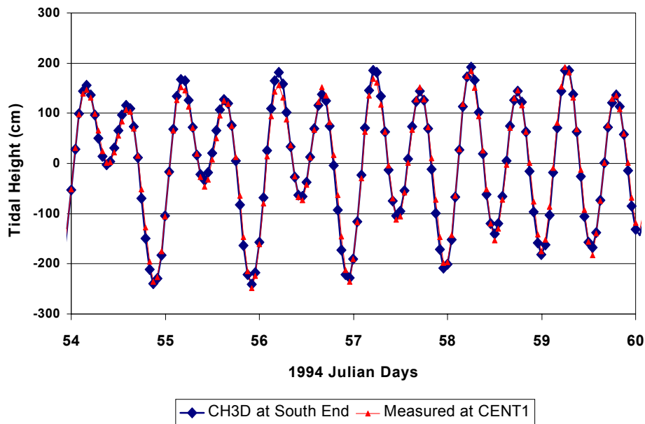
Figure 8b. Comparison of tides between CH3D-prediction and measurement
