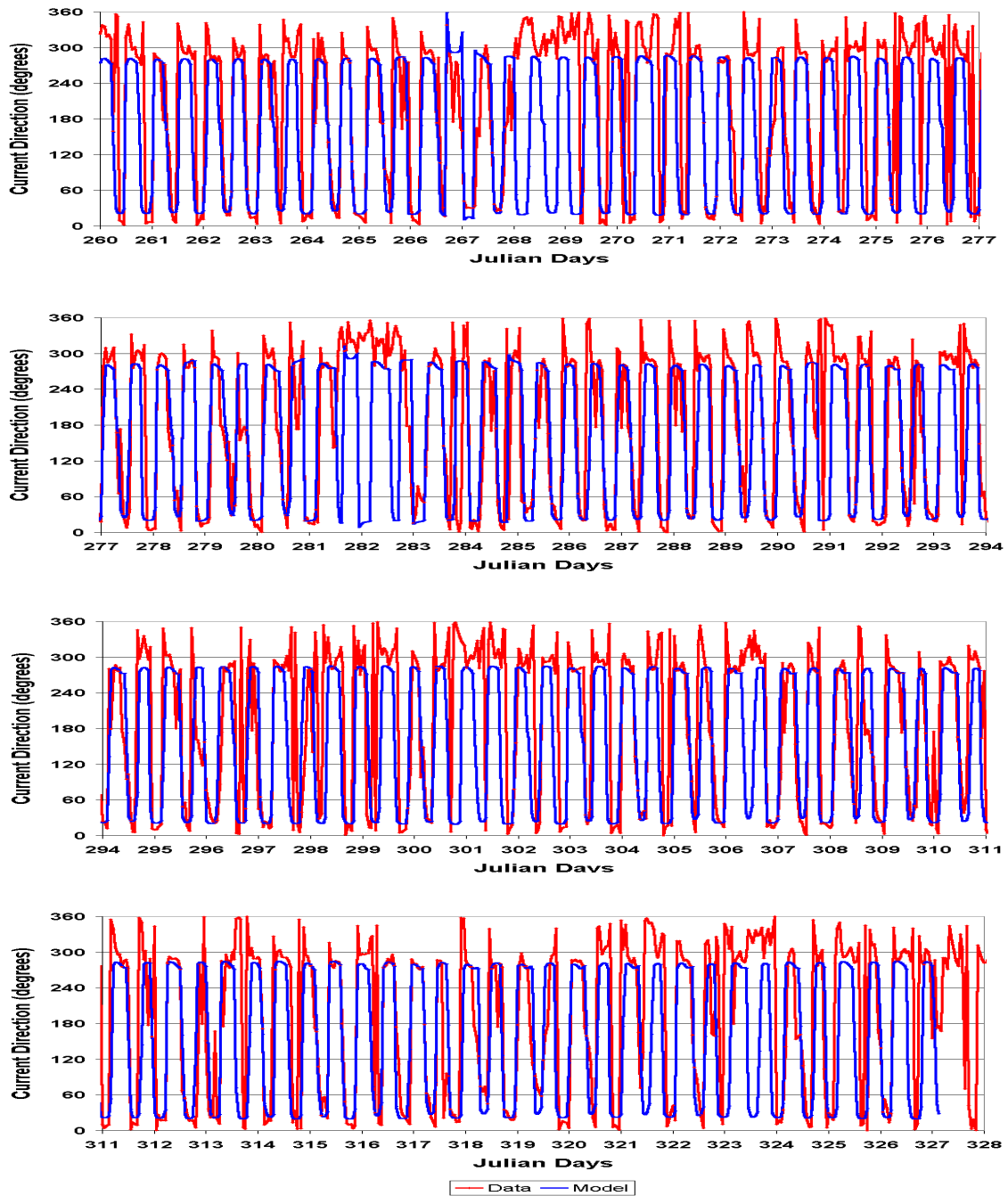
Figure 15b. Comparisons of predicted and measured current directions at SPA1
