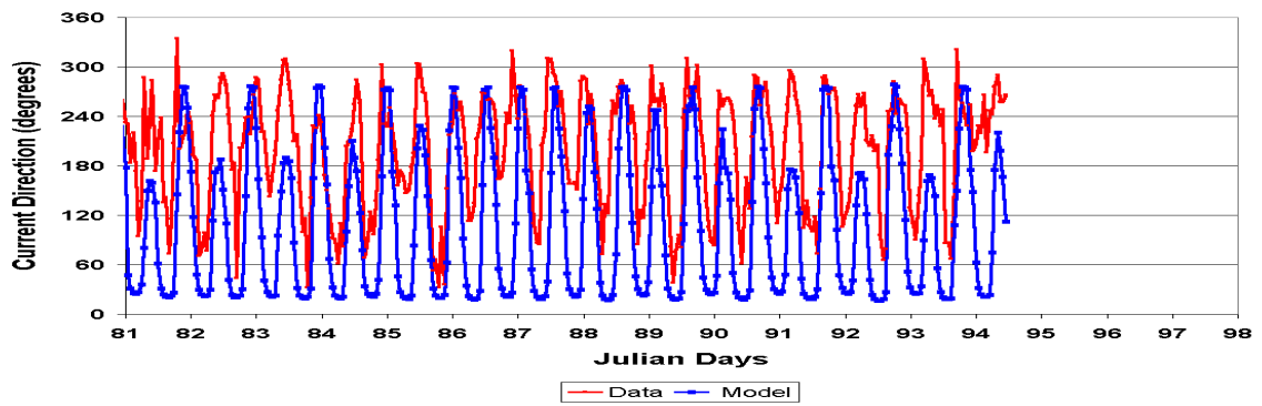
Figure 11b. Comparison of predicted and measured current directions at WEST1
