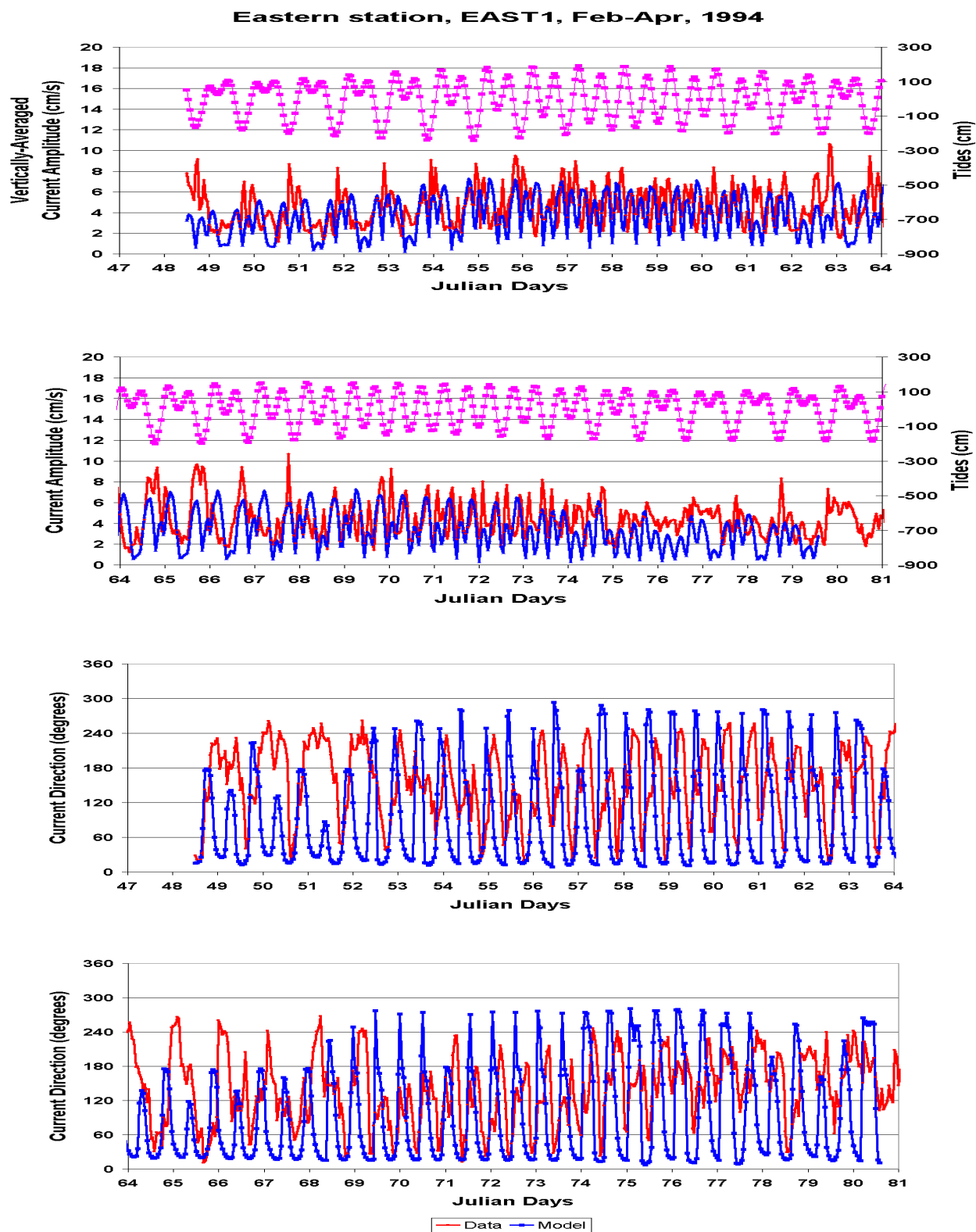
Figure 10. Comparison of predicted and measured current amplitudes and directions at EAST1
