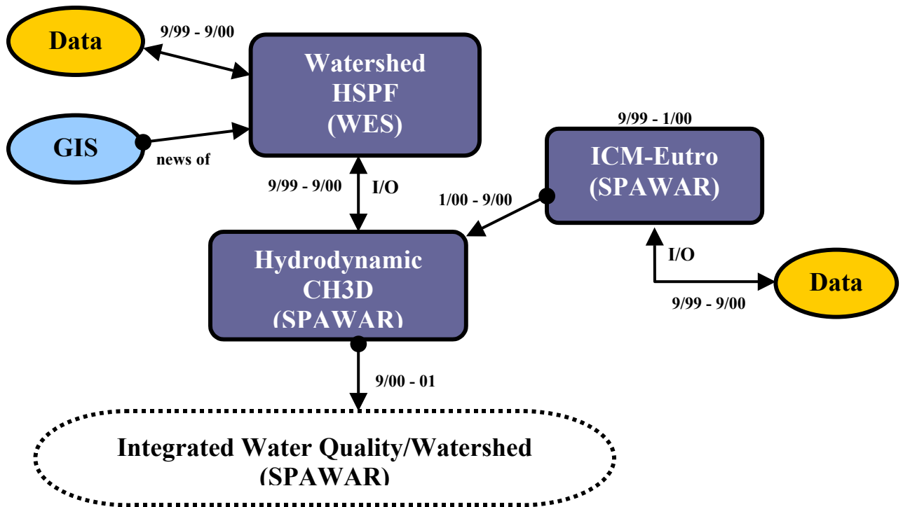
Figure 22. Flow chart and schedules of the linked watershed model for Sinclair Inlet
