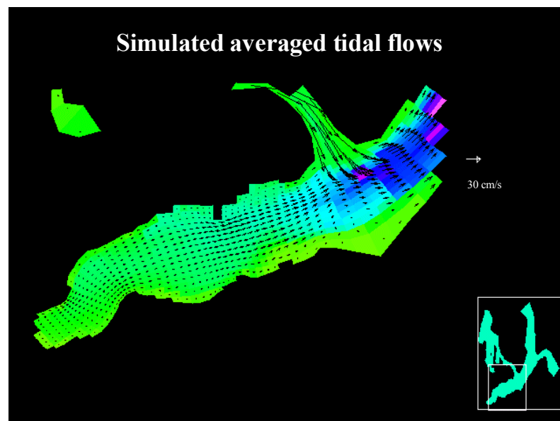
Figure 21a. Gyres at the mouth during ebbing tides
