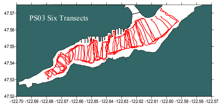
Figure 6. Typical trajectory of boat measuring water-column currents
