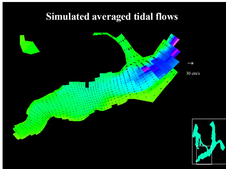
Figure 21b. Gyres at the mouth during slack water
