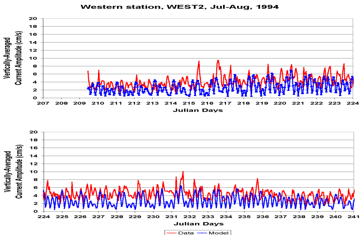
Figure 14a. Comparisons of predicted and measured current amplitudes at WEST2
