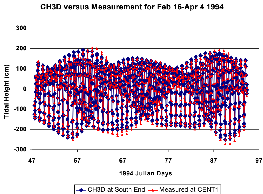
Figure 8a. Comparison of tides between CH3D-prediction and measurement
