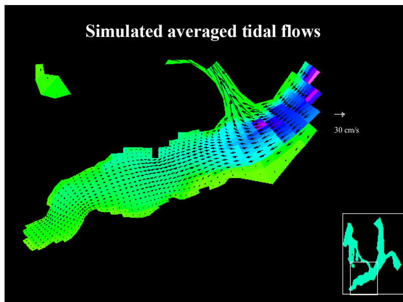
Figure 21c. Gyres at the mouth during flooding water
