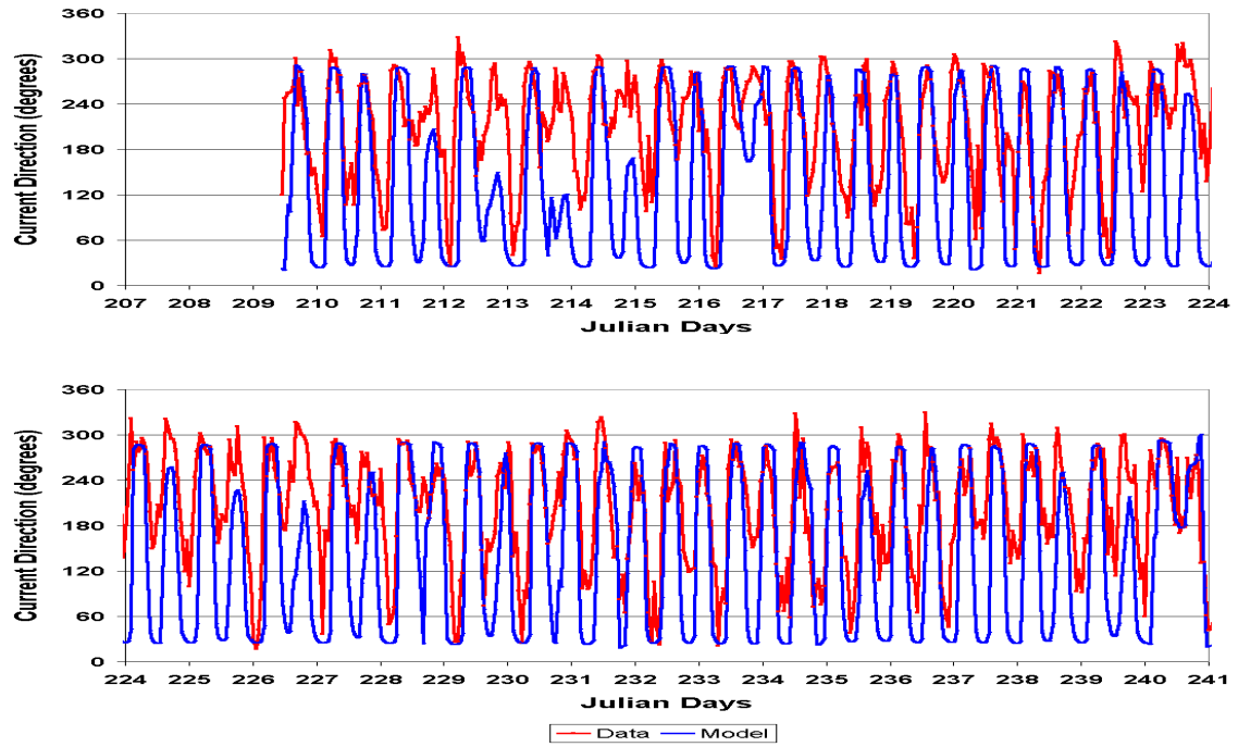
Figure 14c. Comparisons of predicted and measured current directions at WEST2
