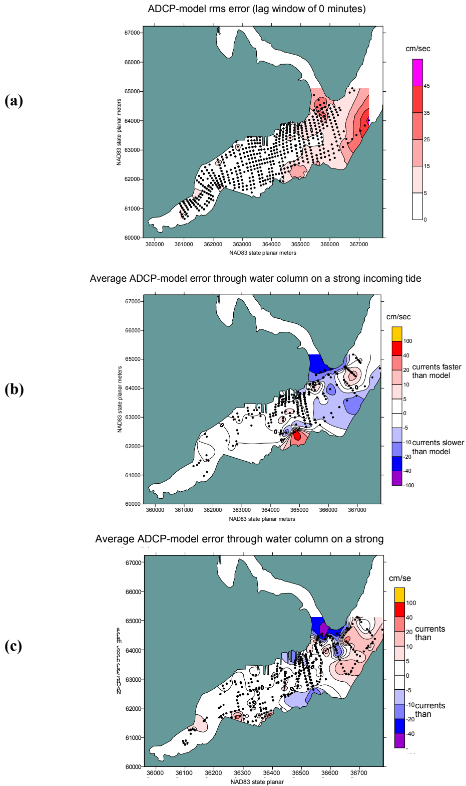
Figure 17. Root-Mean-Square errors of currents between measurement and model for (a) average tidal condition, (b) flood tides and (c) ebb tides
