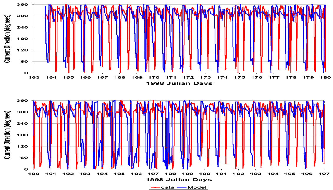
Figure 16b. Comparisons of predicted and measured current directions at SPA2
