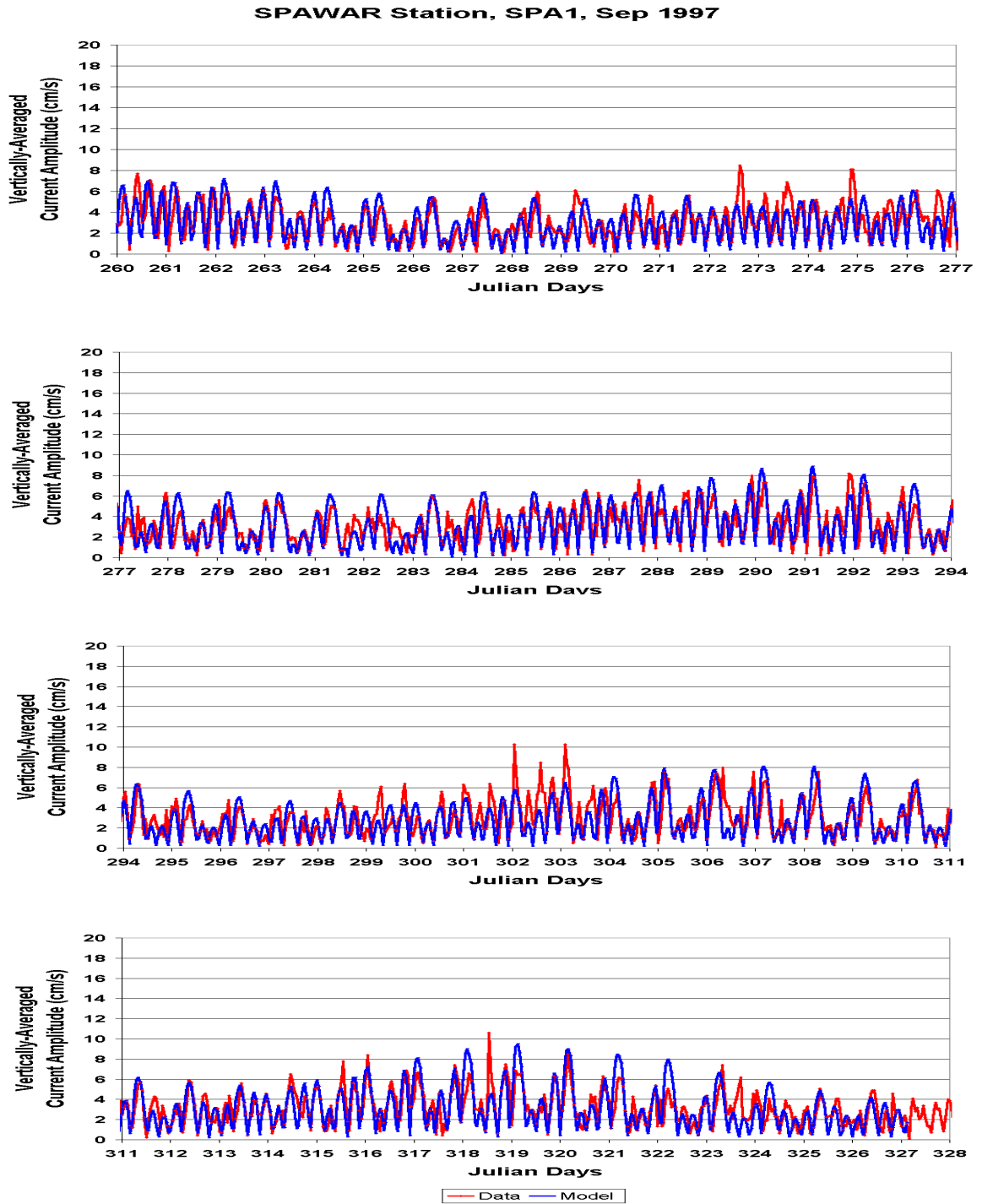
Figure 15a. Comparisons of predicted and measured current amplitudes at SPA1
