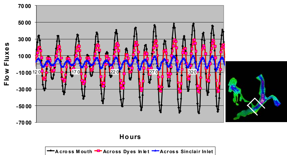
Figure 19. Tidal flow fluxes across Port Orchard Passage, Dyes Inlet and Sinclair Inlet
