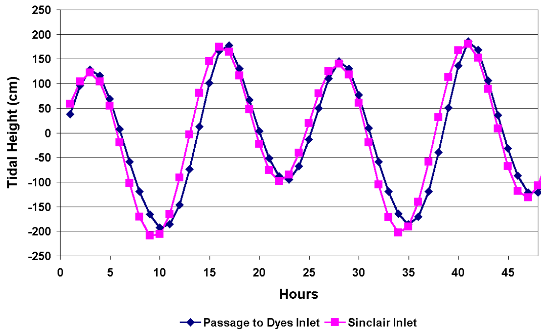
Figure 20. Tides with phase difference between Dyes Inlet and Sinclair Inlet
