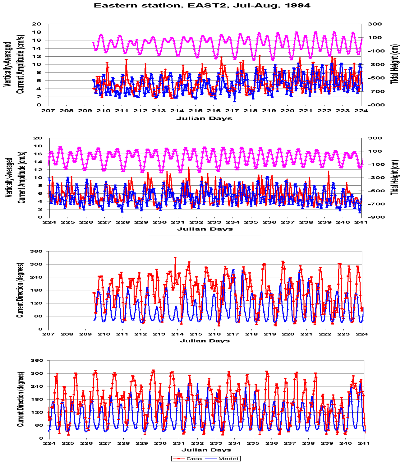
Figure 13. Comparisons of predicted and measured current amplitudes and directions at EAST2
