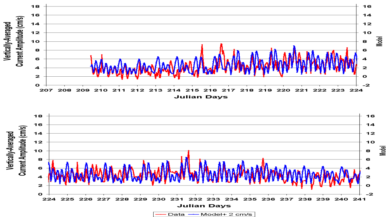
Figure 14b. Comparisons of measured and (predicted + 2 cm/s) current amplitudes at WEST2
