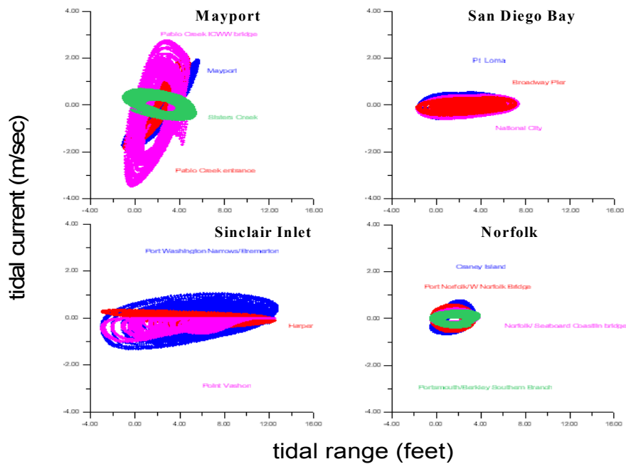
Figure 18. Current-tide relationships for 4 navy harbors
