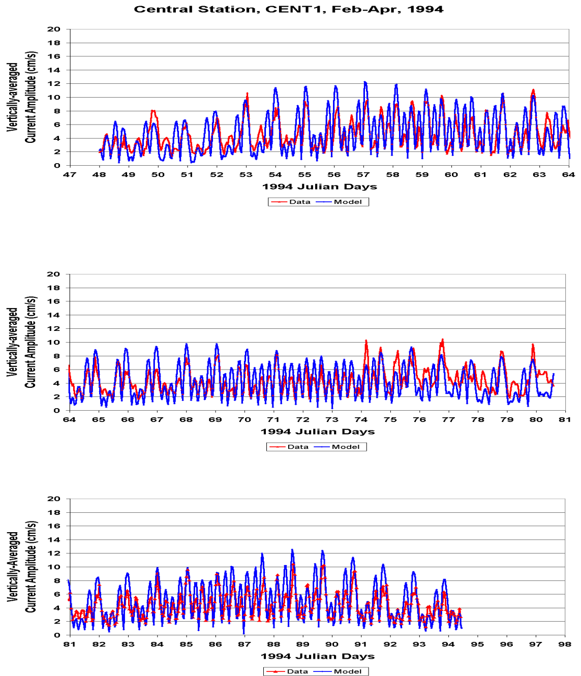
Figure 9a. Comparison of predicted and measured current amplitudes at CENT1
