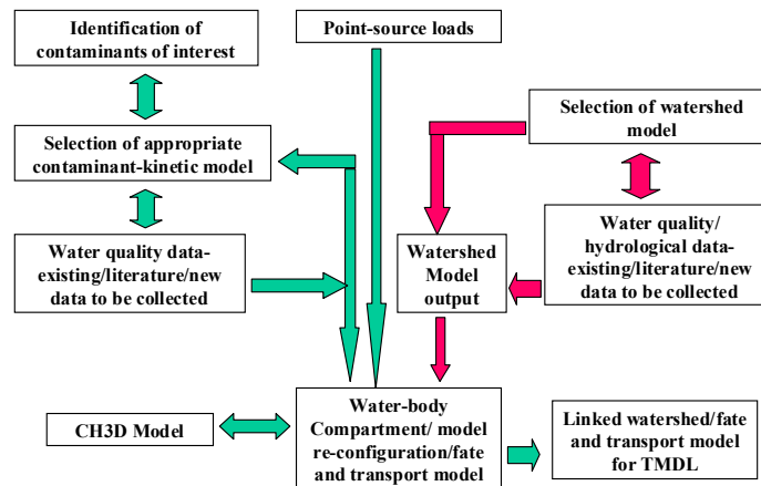
Figure 2. Linked watershed modeling framework of TMDL for Sinclair Inlet
