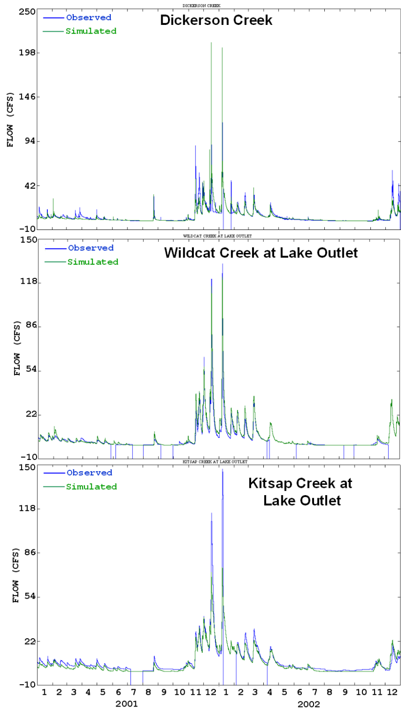
Figure 2-4. Observed and simulated 15-minute flows used for calibrating subwatersheds in the Chico Creek basin from January 2001 to December 2002.
