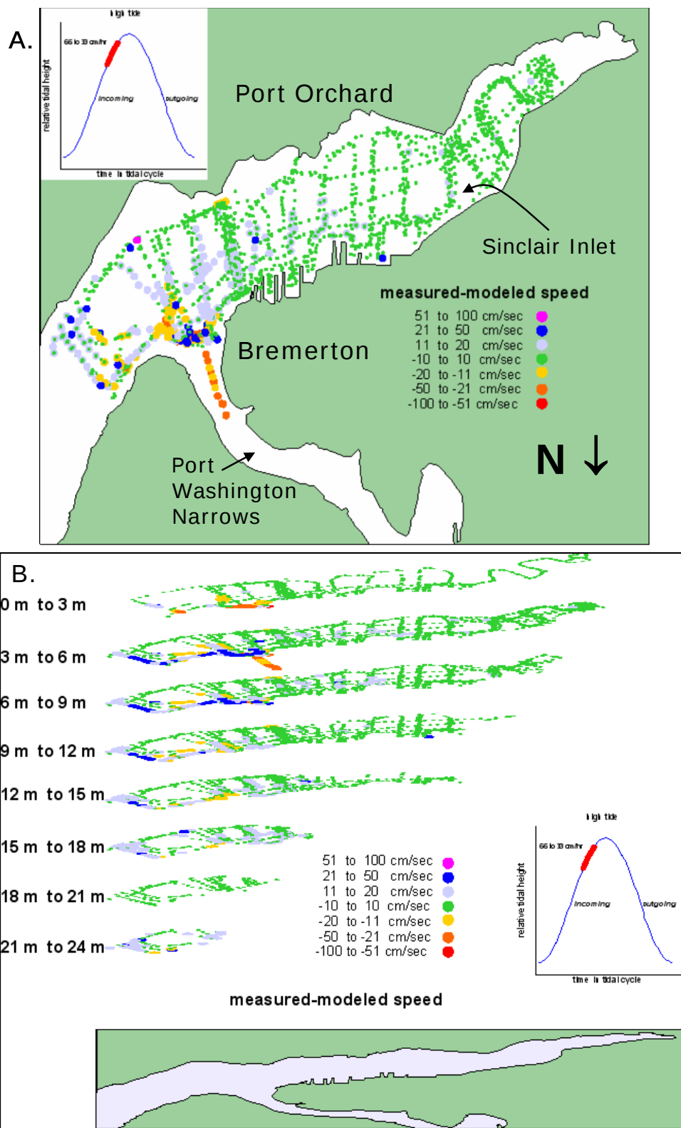
Figure 2-18. Absolute difference between modeled and measured current speed at all depths (A) and horizontally smoothed and extrapolated absolute difference by depth (B) during tide condition 5 (end of flood) based on 3859 observations (from Richter, 2004).
