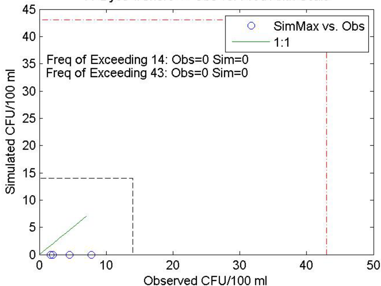
11-Dyes-wShore---- Obs vs. Pred Arith Scale
