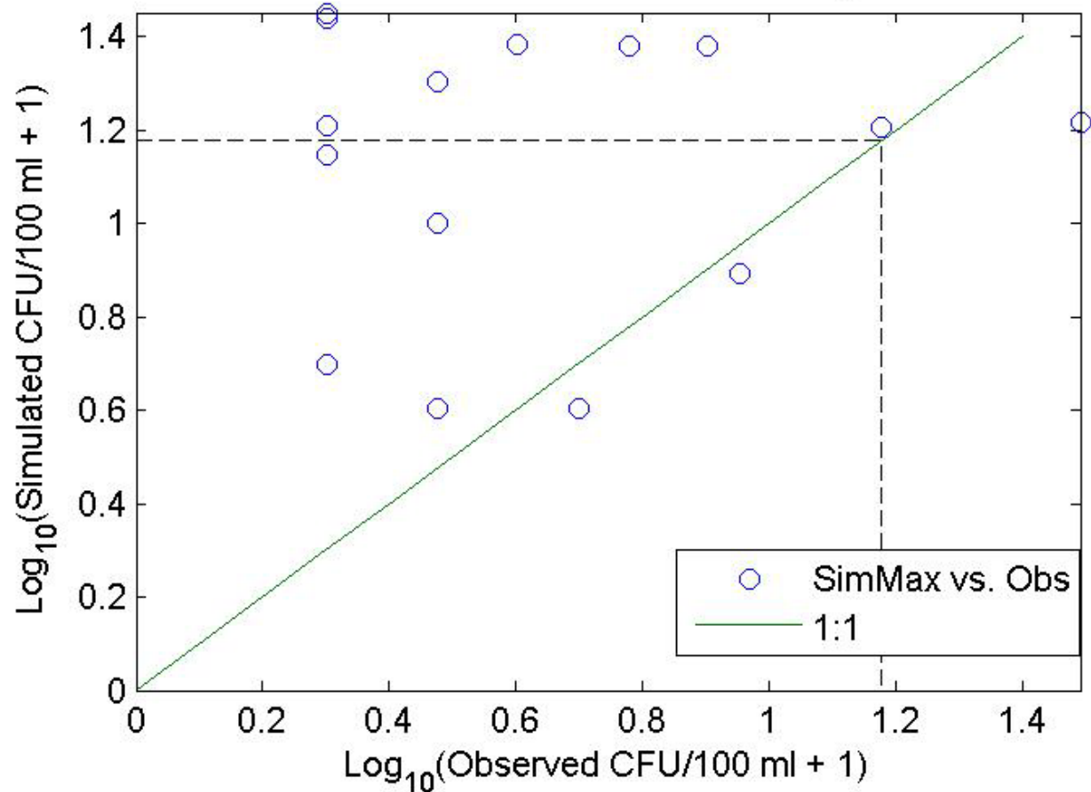
43-Sin-Gorst-Creek Obs vs. Pred Log Scale
