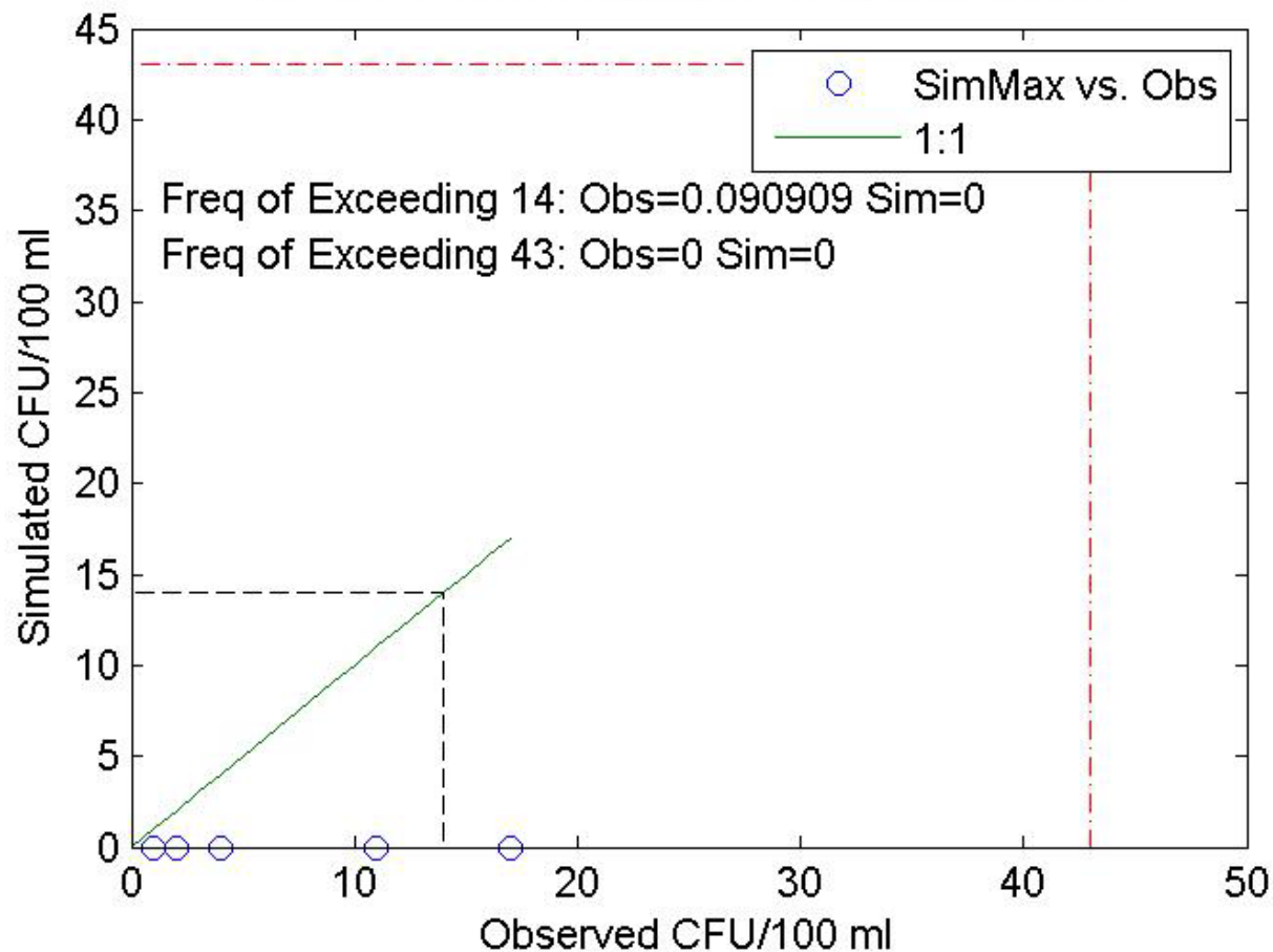
18-POP-SN17-Waterm Obs vs. Pred Arith Scale
