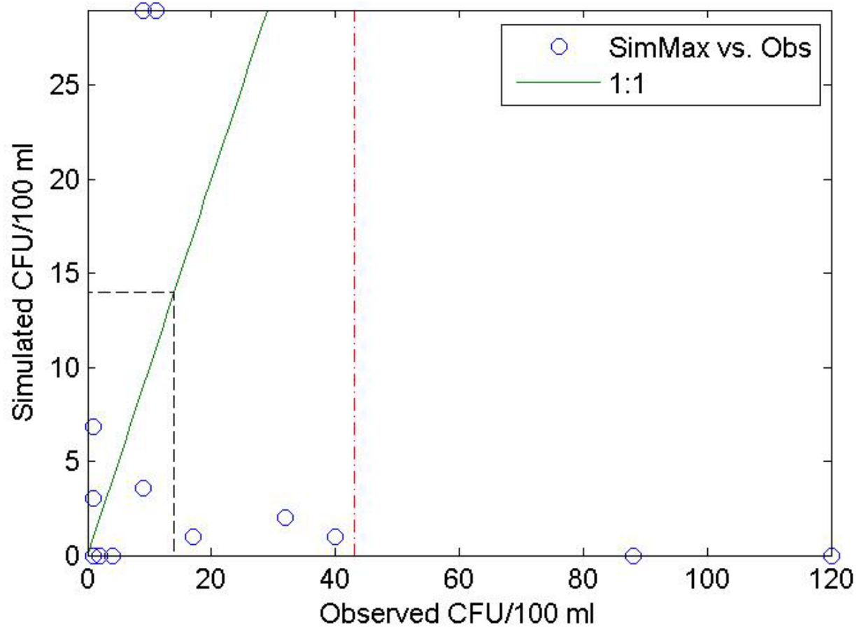
51-SinPO-KarcherCr Obs vs. Pred Arith Scale
