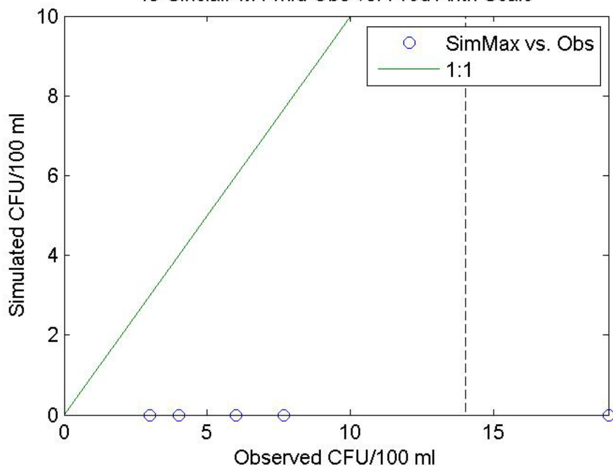
45-Sinclair-M4-mid Obs vs. Pred Arith Scale
