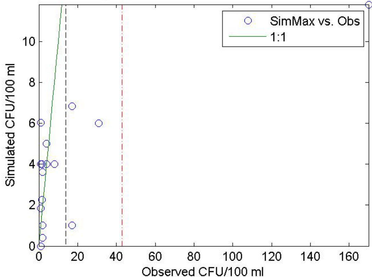
04-Dyes-DY24-Straw Obs vs. Pred Arith Scale
