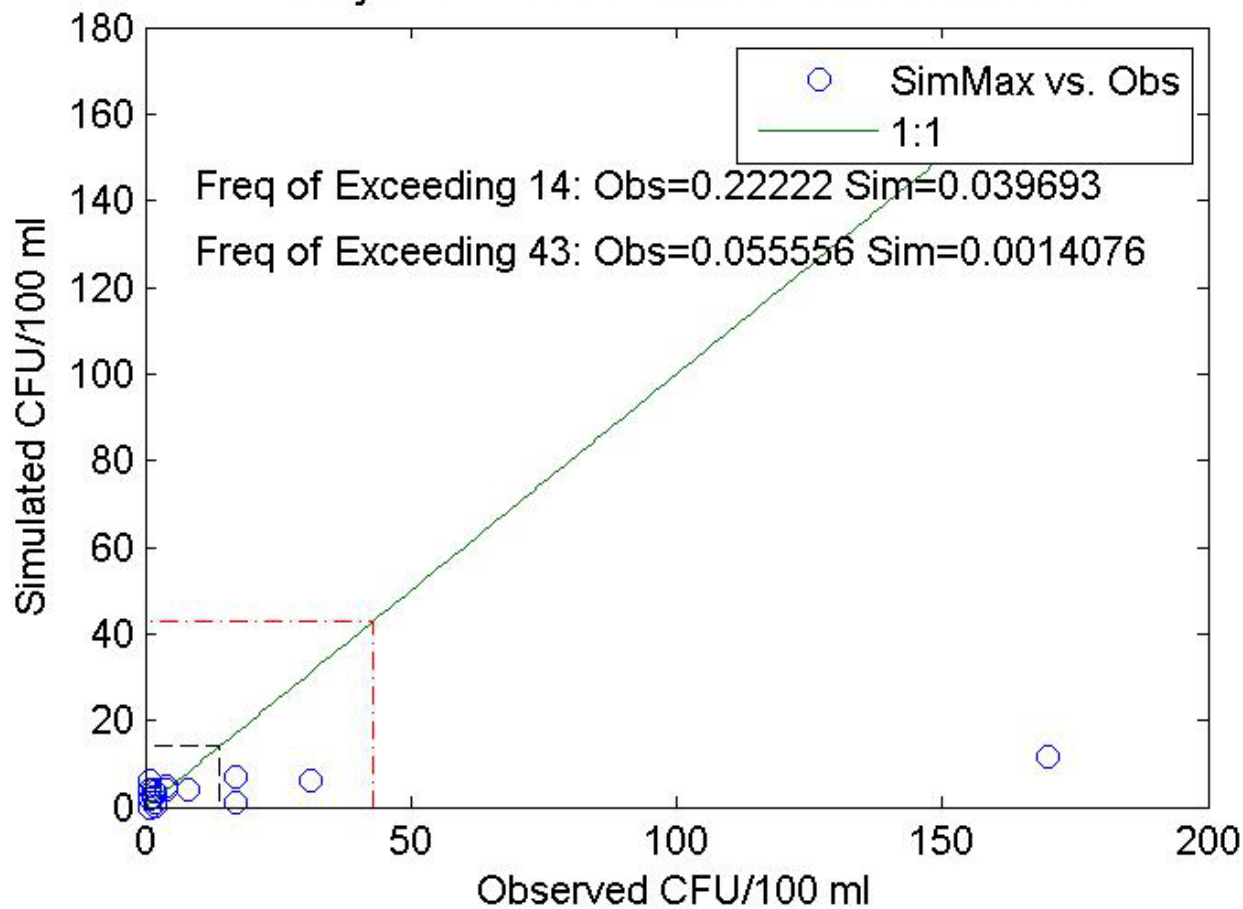
04-Dyes-DY24-Straw Obs vs. Pred Arith Scale
