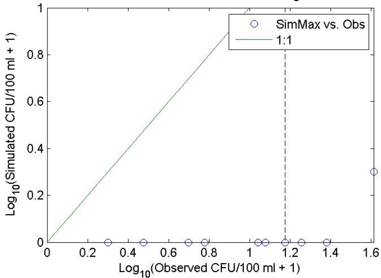
52-SinPO-SN10-wfro Obs vs. Pred Log Scale
