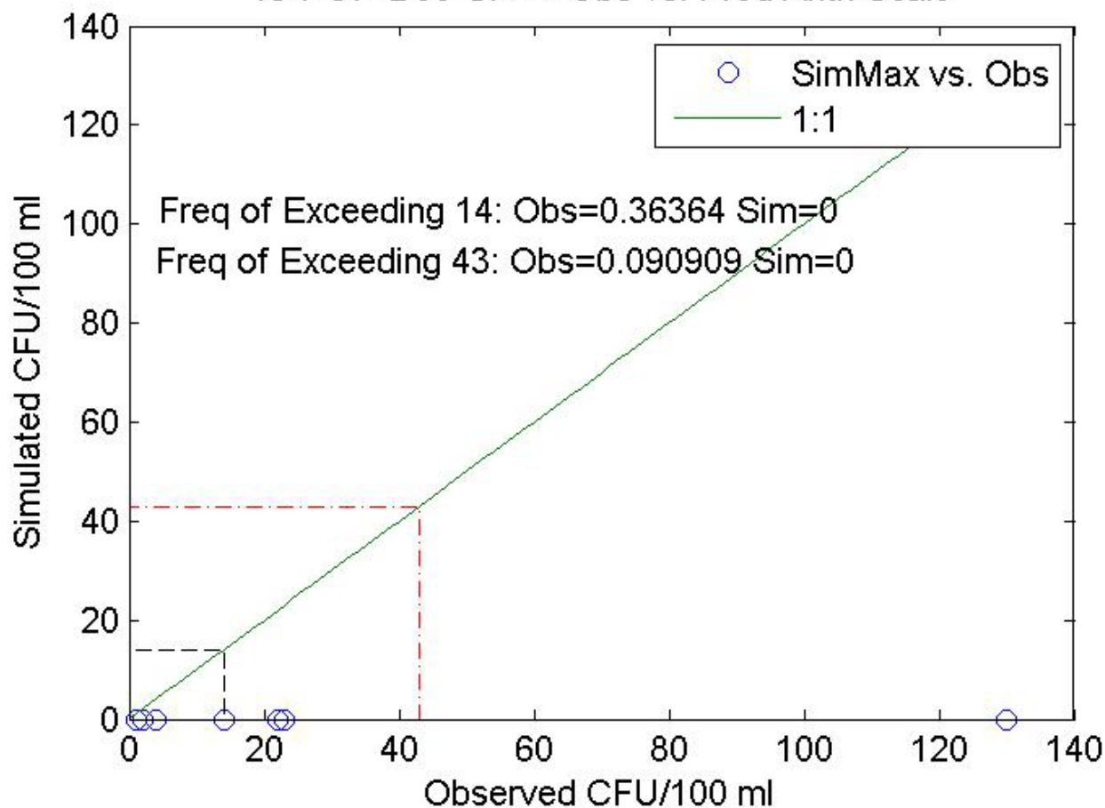
19-POP-Dee-Cr---- Obs vs. Pred Arith Scale
