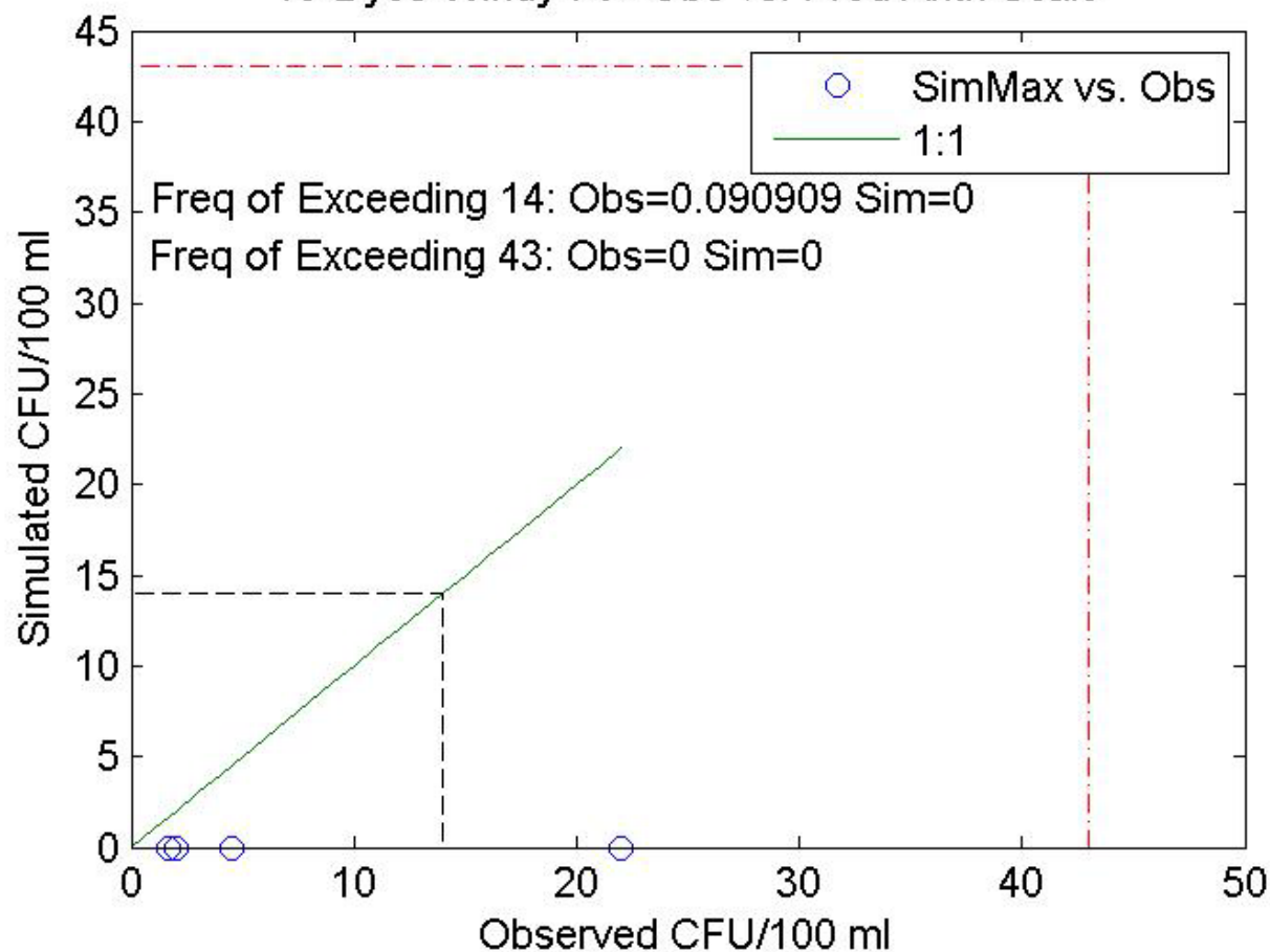
10-Dyes-Windy-Pt-- Obs vs. Pred Arith Scale
