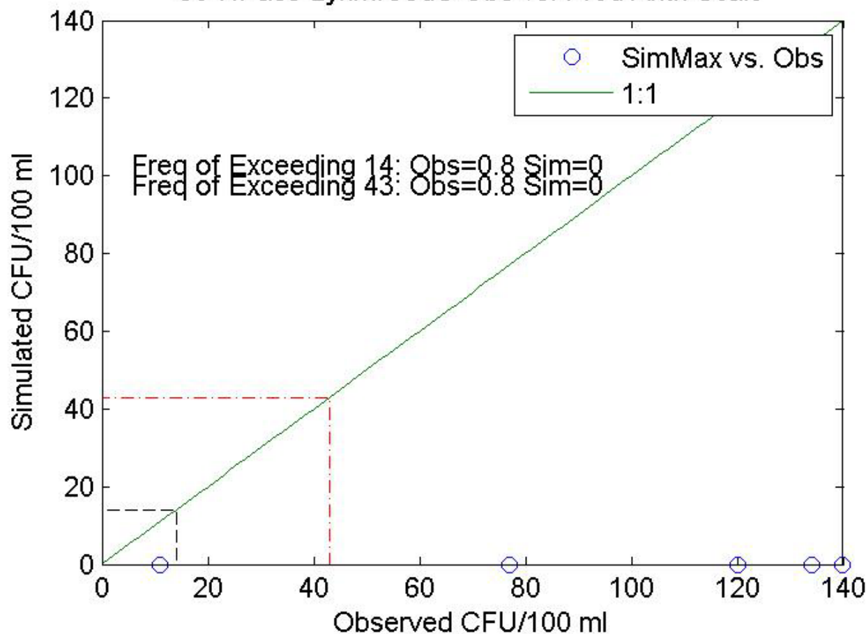
36-RPass-LynhwoodC Obs vs. Pred Arith Scale
