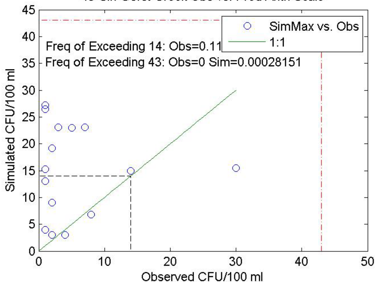
43-Sin-Gorst-Creek Obs vs. Pred Arith Scale
