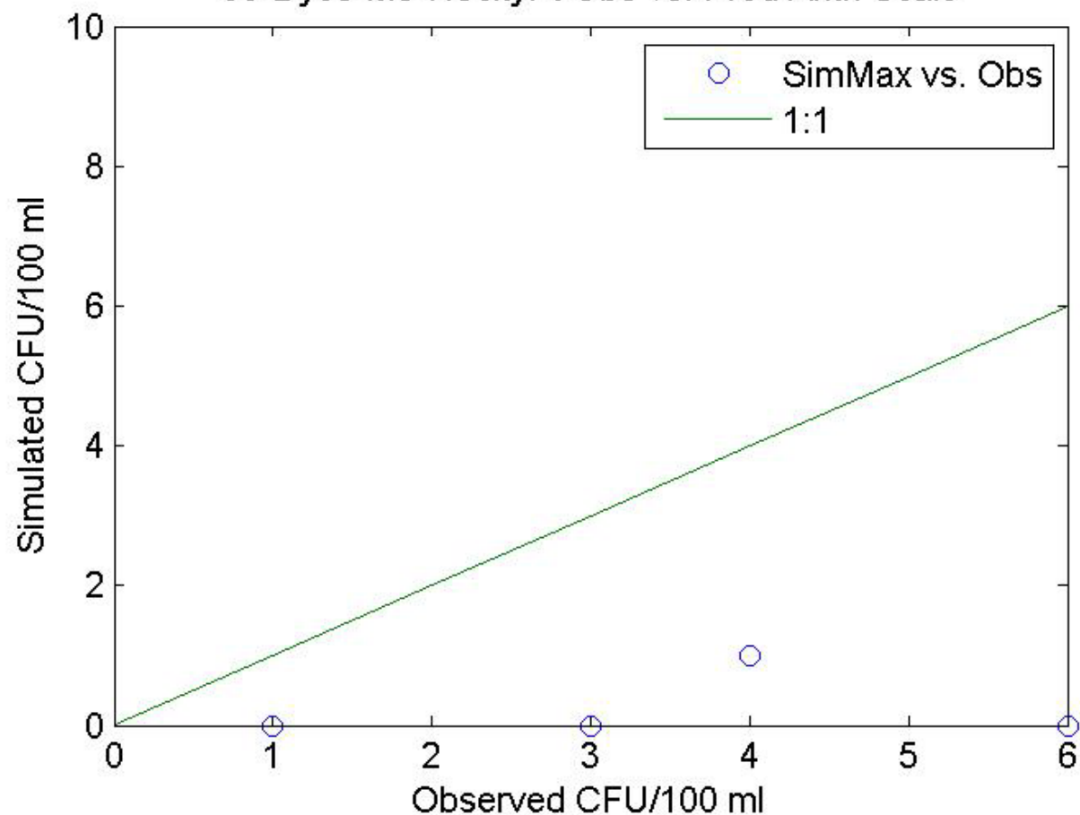
08-Dyes-M5-RockyPt Obs vs. Pred Arith Scale
