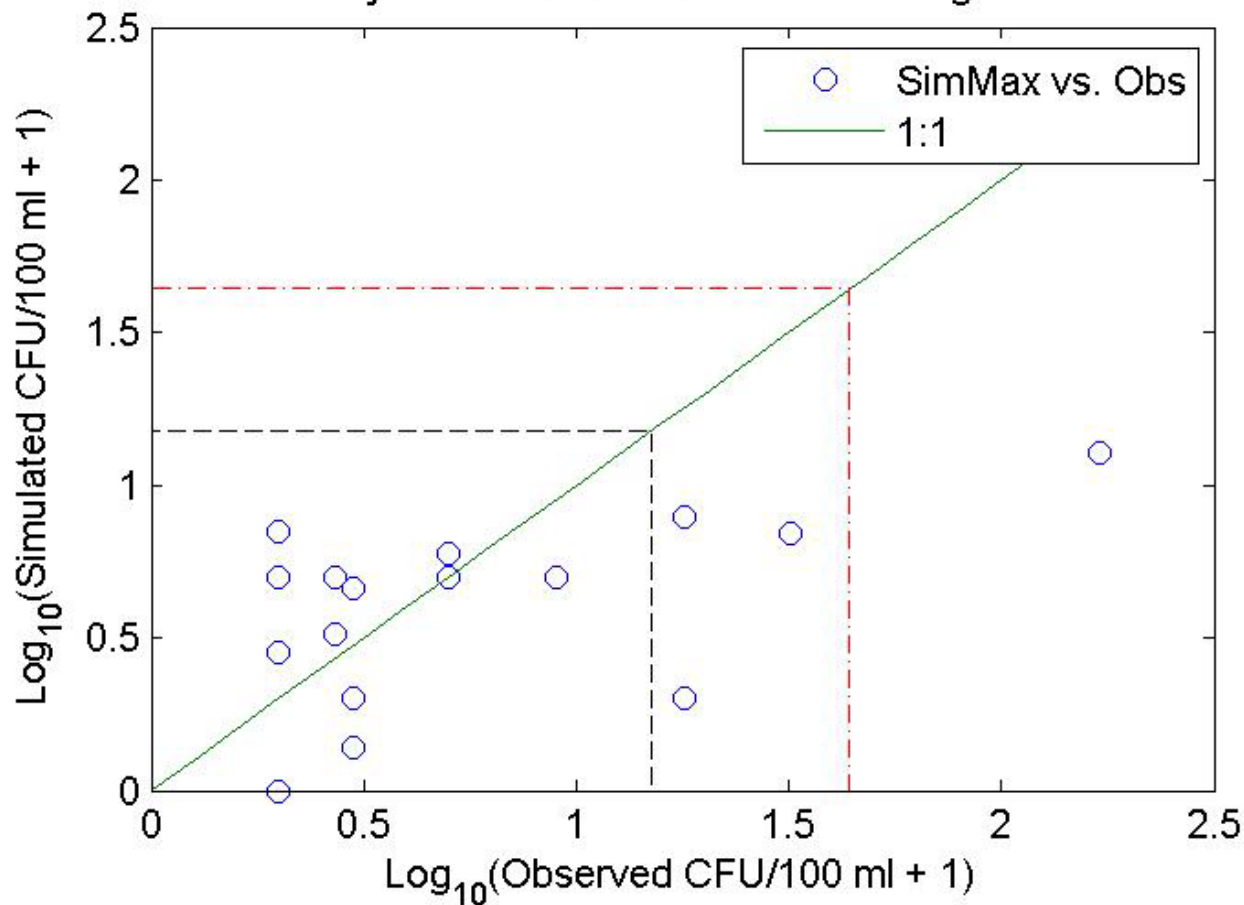
04-Dyes-DY24-Straw Obs vs. Pred Log Scale
