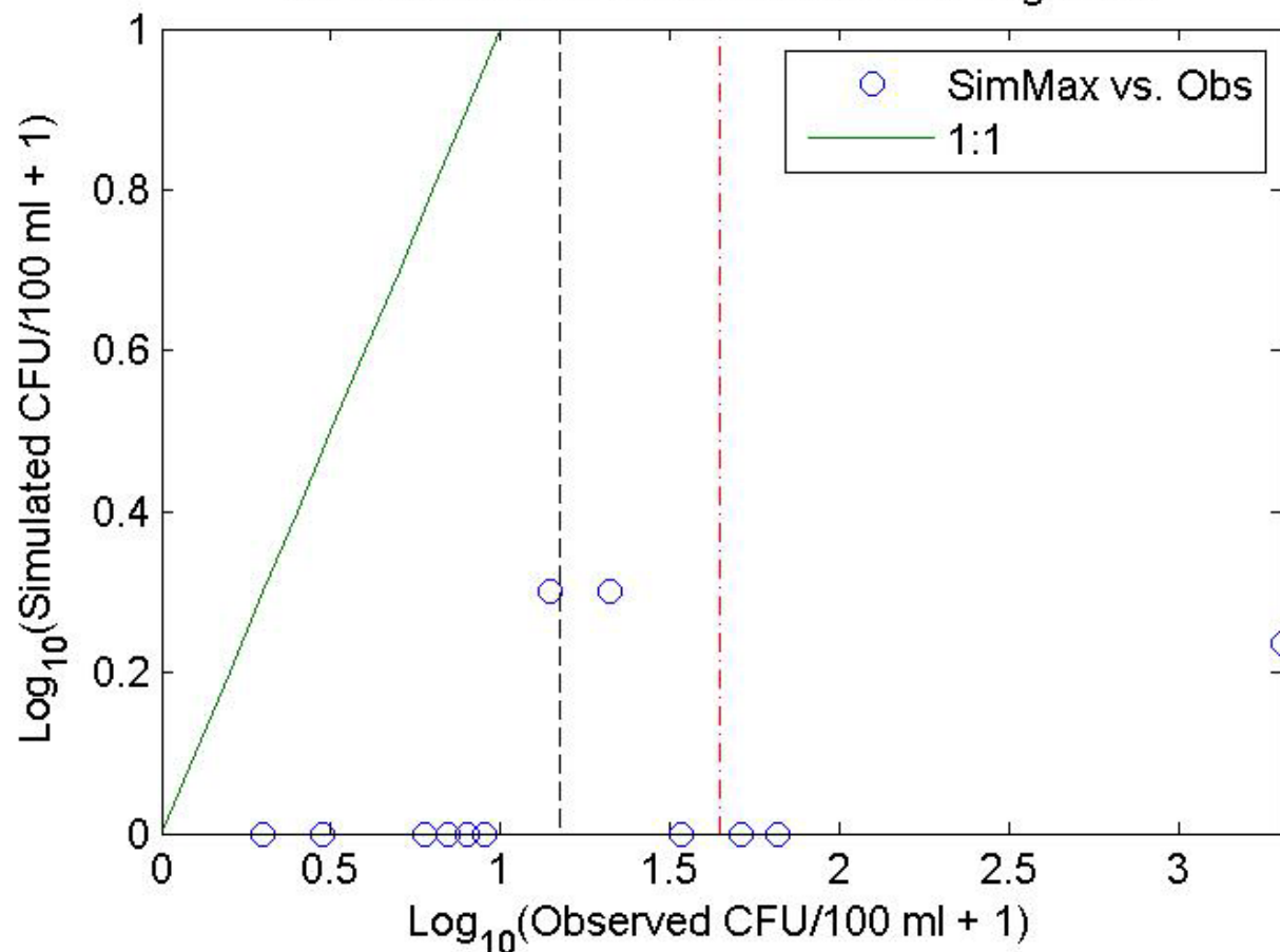
33-PWN-AnCov-PineR Obs vs. Pred Log Scale
