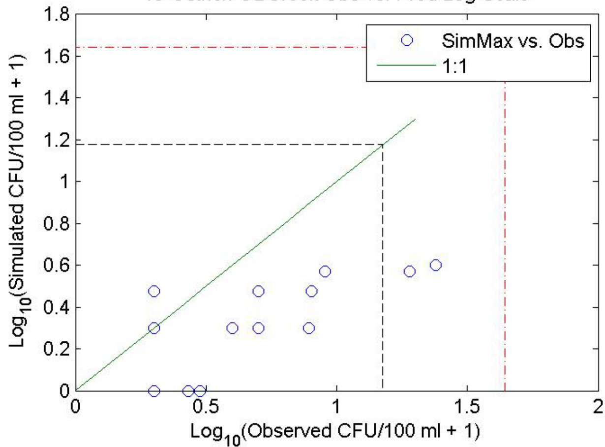
15-Ostrich-OBCreek Obs vs. Pred Log Scale
