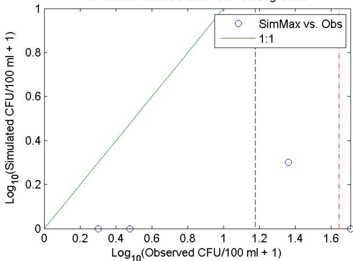
48-Sinclair-SaccoC Obs vs. Pred Log Scale
