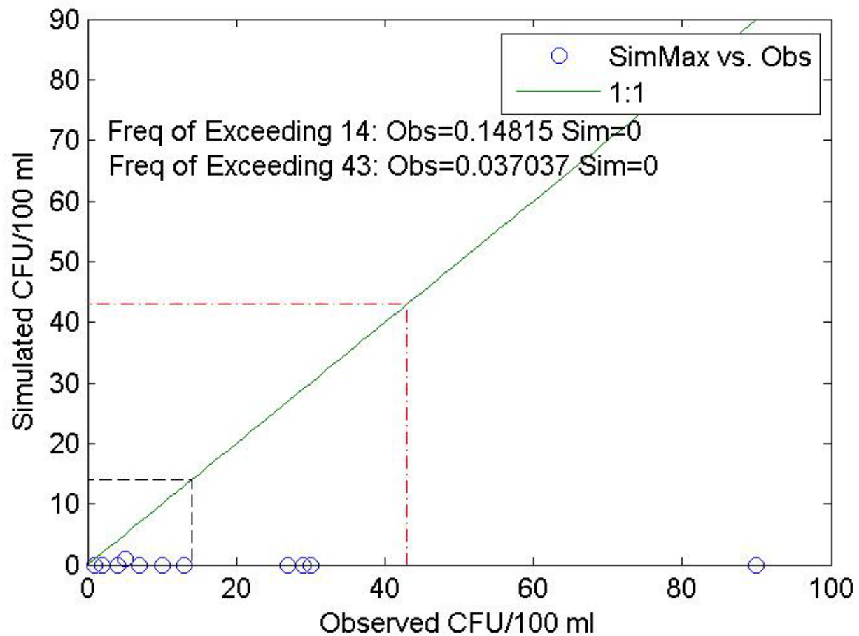
53-Sin-SN11-12mari Obs vs. Pred Arith Scale
