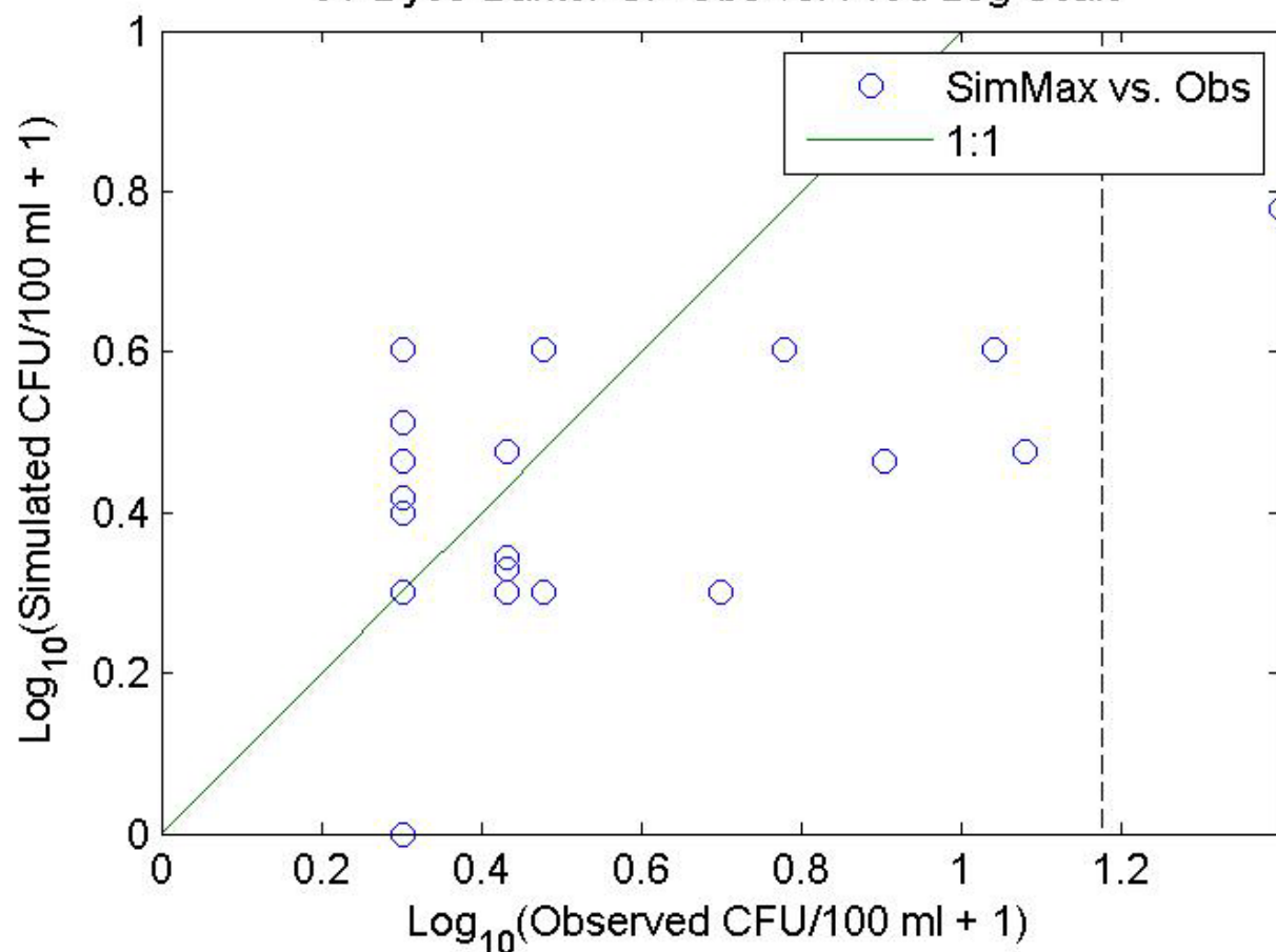
01-Dyes-Barker-Cr- Obs vs. Pred Log Scale
