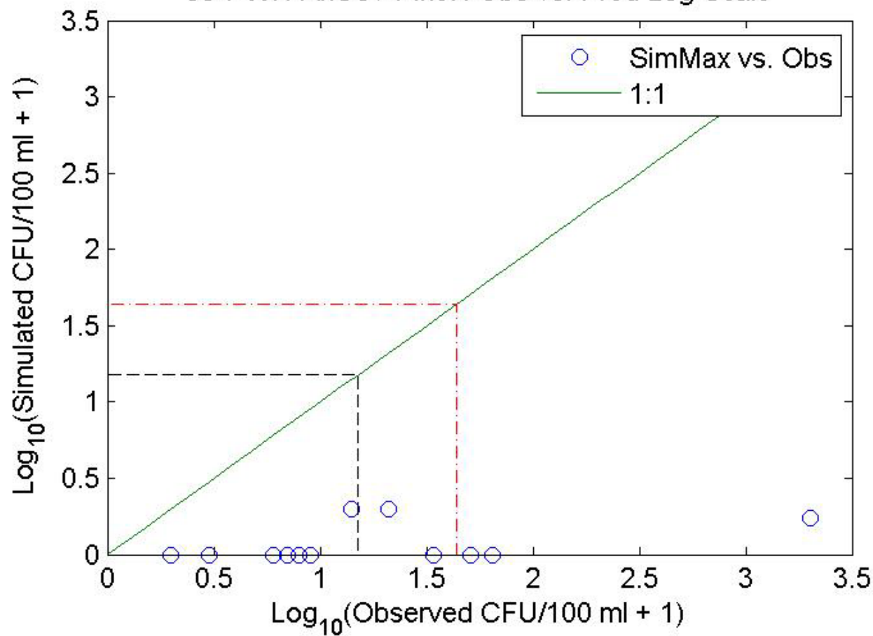
33-PWN-AnCov-PineR Obs vs. Pred Log Scale
