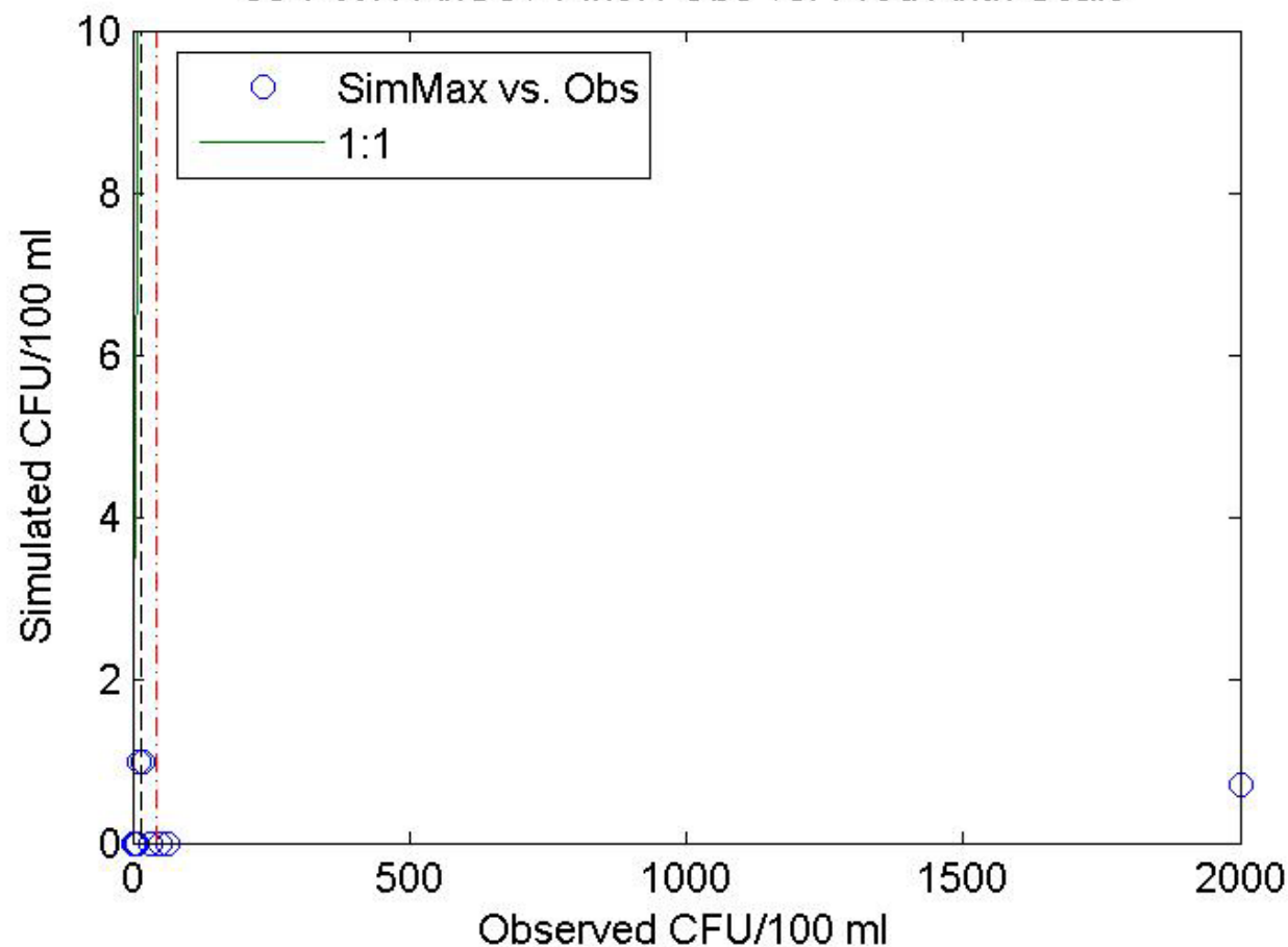
33-PWN-AnCov-PineR Obs vs. Pred Arith Scale
