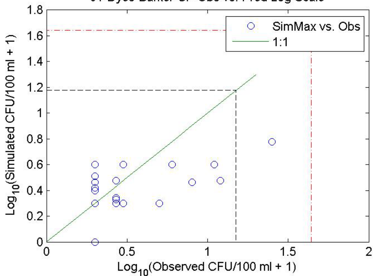
01-Dyes-Barker-Cr- Obs vs. Pred Log Scale
