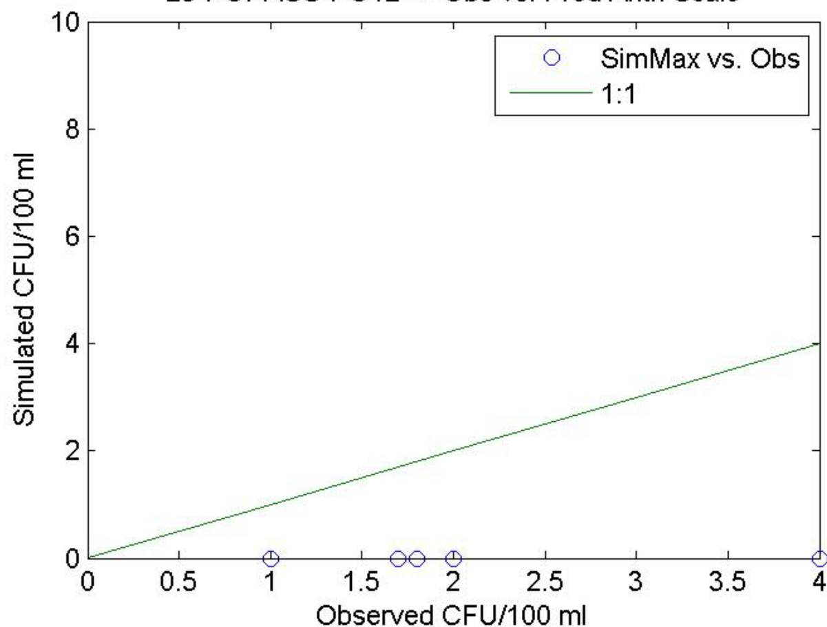
23-POPASS-PO12---- Obs vs. Pred Arith Scale
