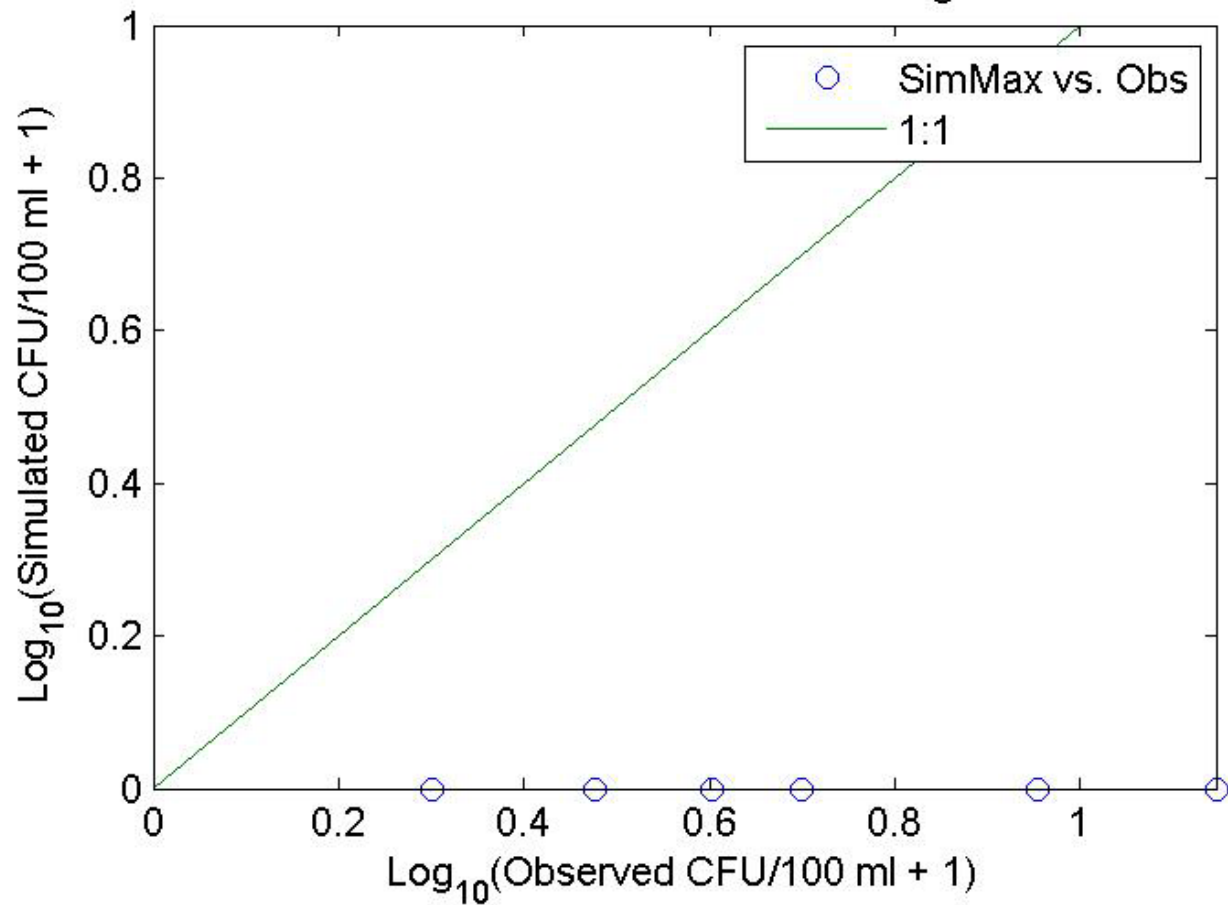
44-Sinclair-M3-mid Obs vs. Pred Log Scale
