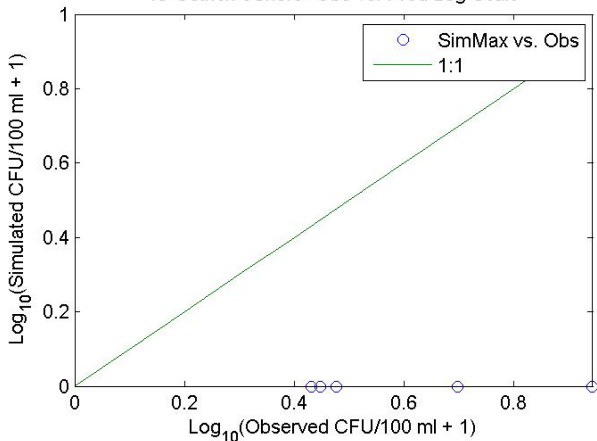
13-Ostrich-eShore- Obs vs. Pred Log Scale
