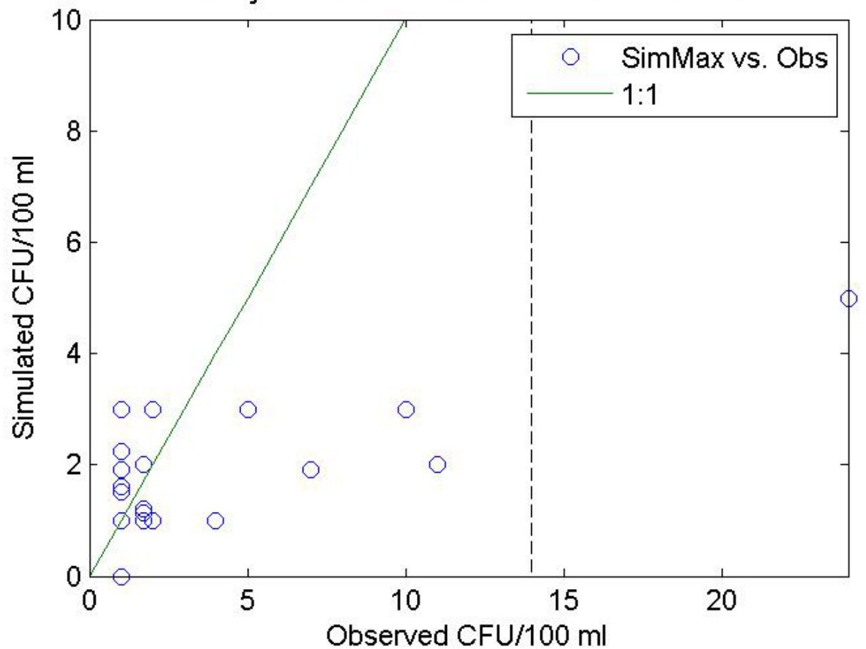
01-Dyes-Barker-Cr- Obs vs. Pred Arith Scale
