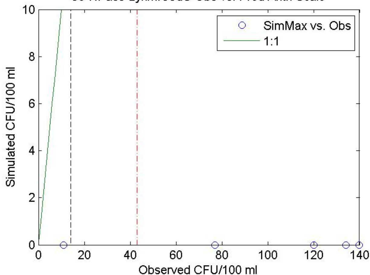
36-RPass-LynhwoodC Obs vs. Pred Arith Scale
