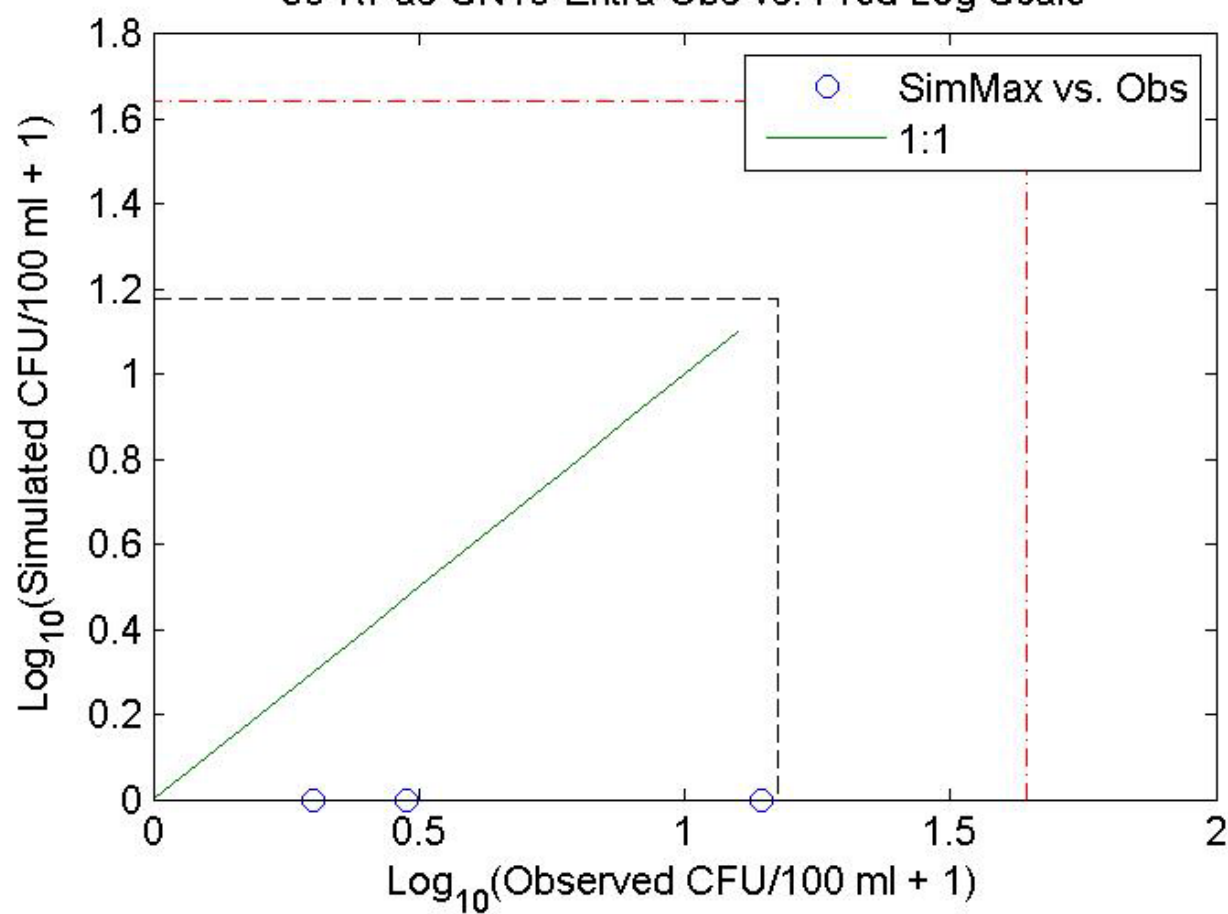
38-RPas-SN18-Entra Obs vs. Pred Log Scale
