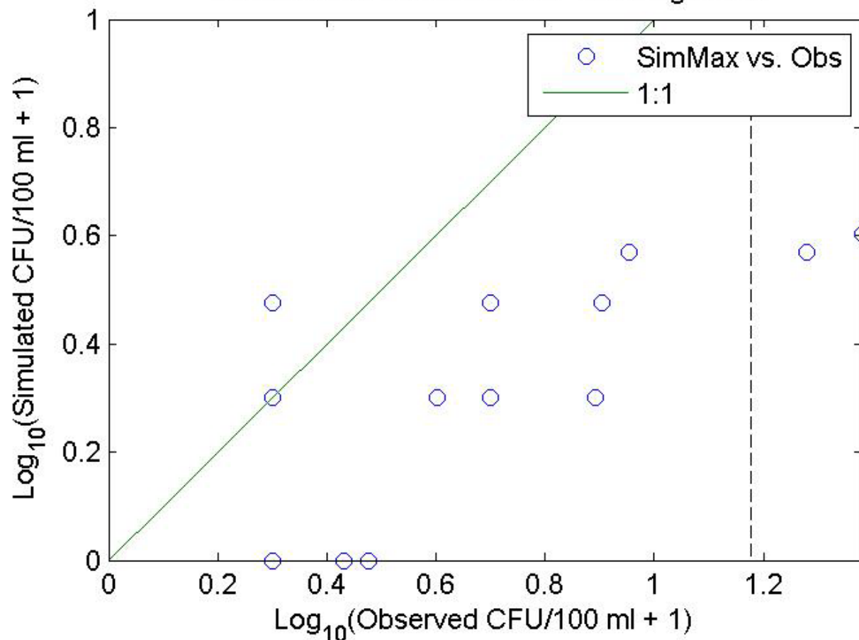
15-Ostrich-OBCreek Obs vs. Pred Log Scale
