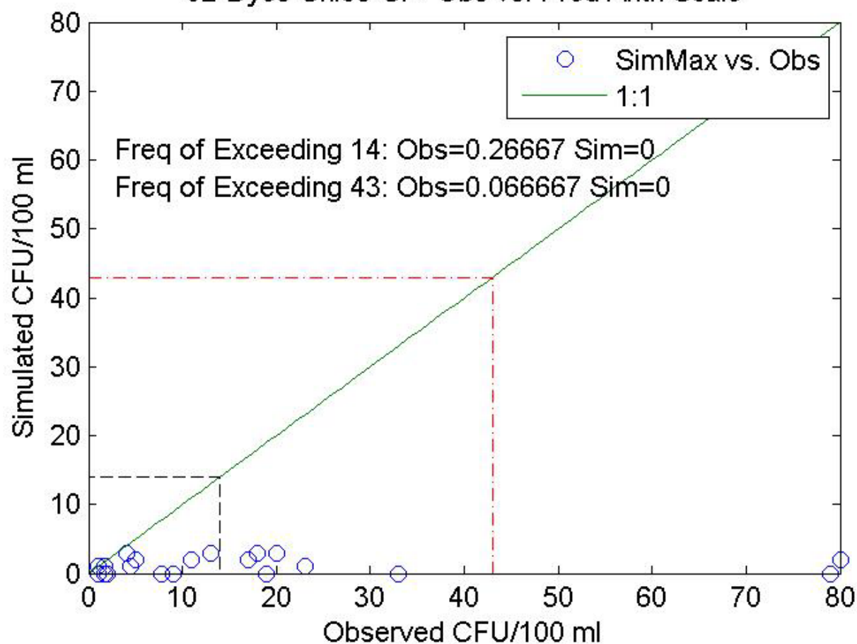
02-Dyes-Chico-Cr-- Obs vs. Pred Arith Scale
