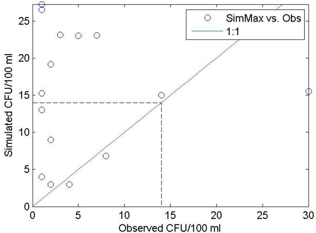
43-Sin-Gorst-Creek Obs vs. Pred Arith Scale
