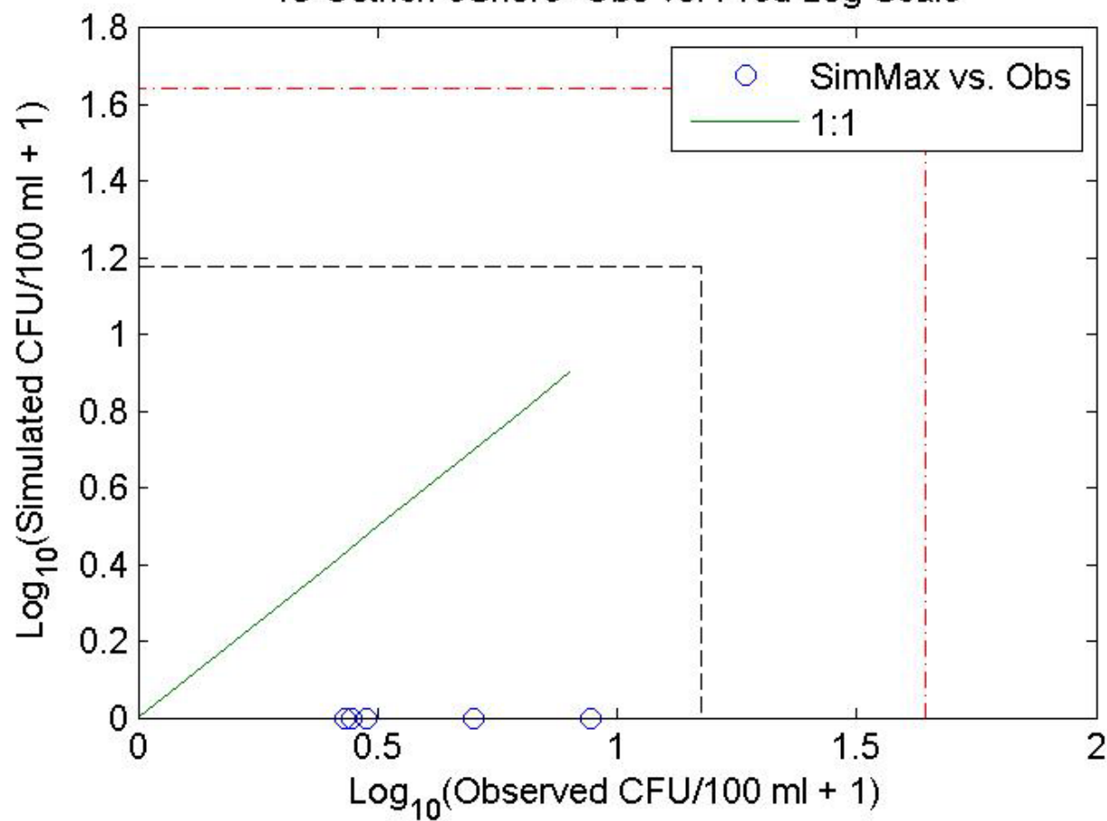
13-Ostrich-eShore- Obs vs. Pred Log Scale
