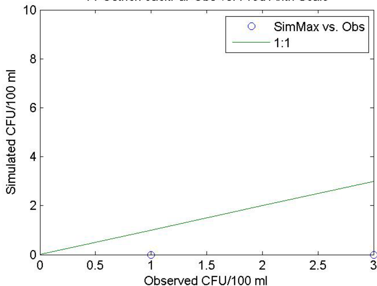
14-Ostrich-JackPar Obs vs. Pred Arith Scale
