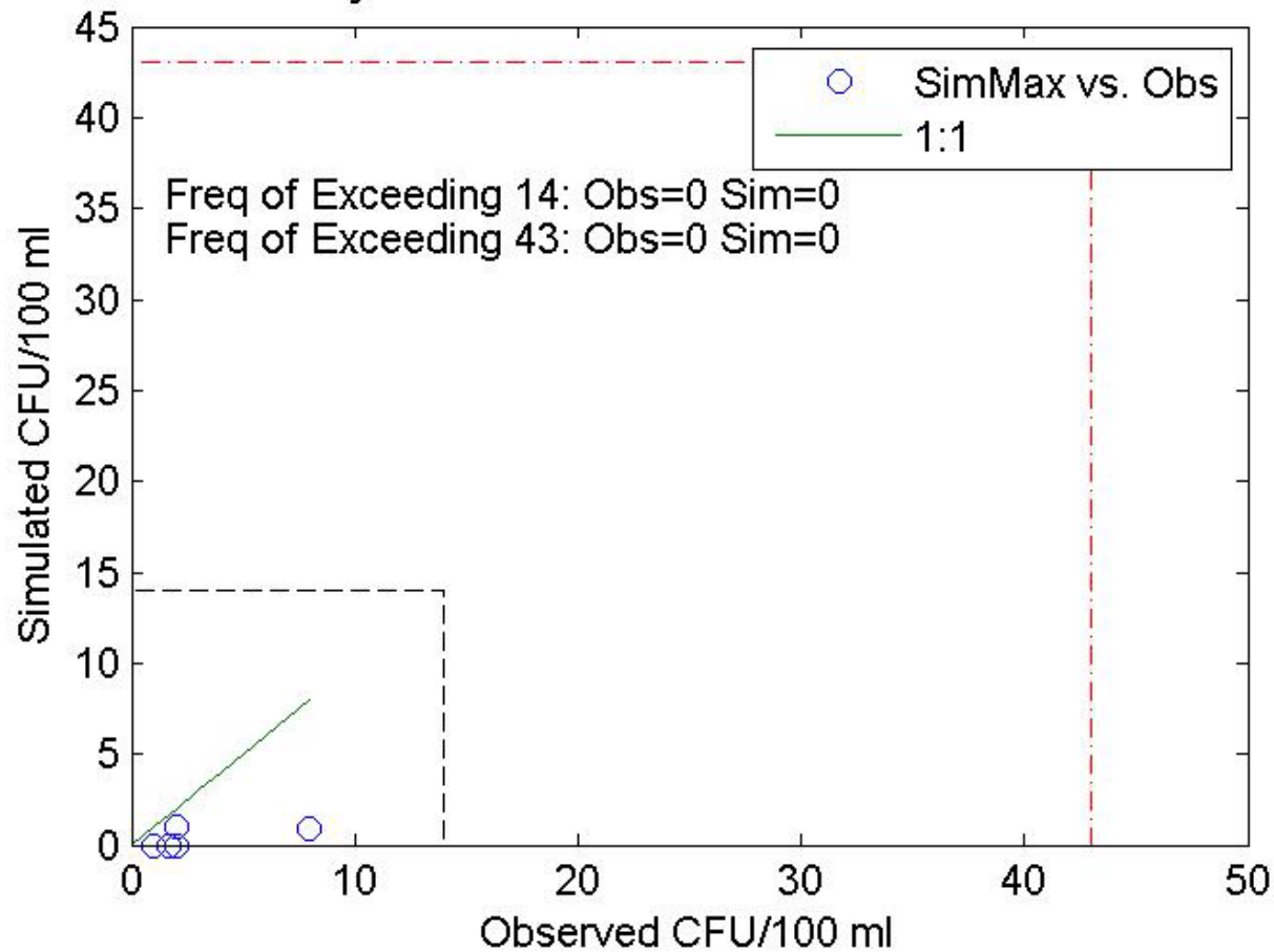
05-Dyes-DY28-Clam Obs vs. Pred Arith Scale
