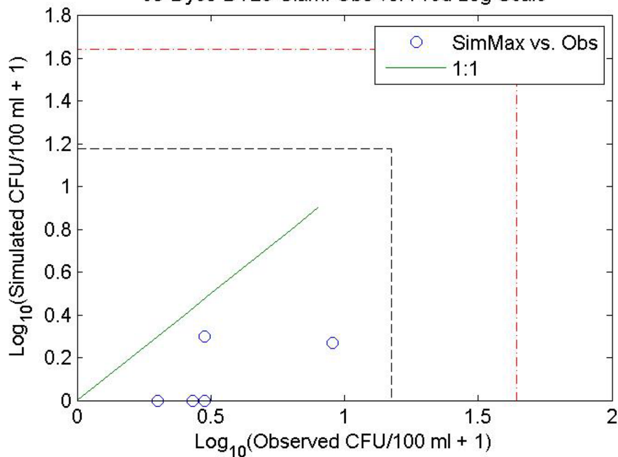
05-Dyes-DY28-Claml Obs vs. Pred Log Scale
