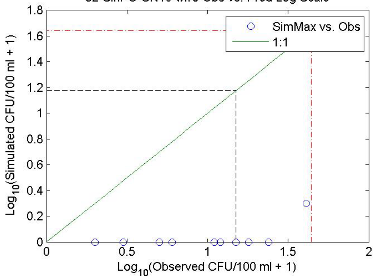
52-SinPO-SN10-wfro Obs vs. Pred Log Scale
