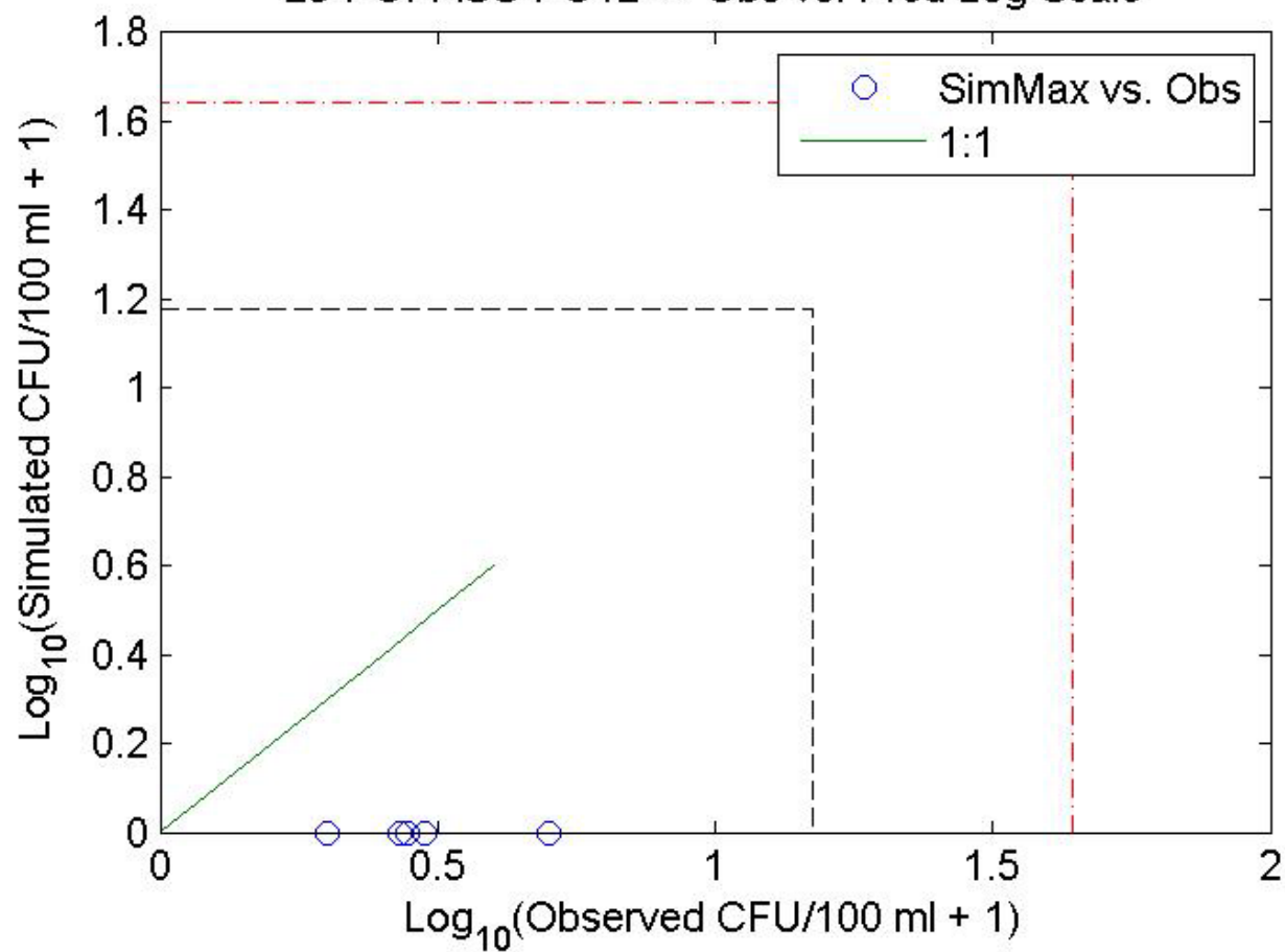
23-POPASS-PO12---- Obs vs. Pred Log Scale
