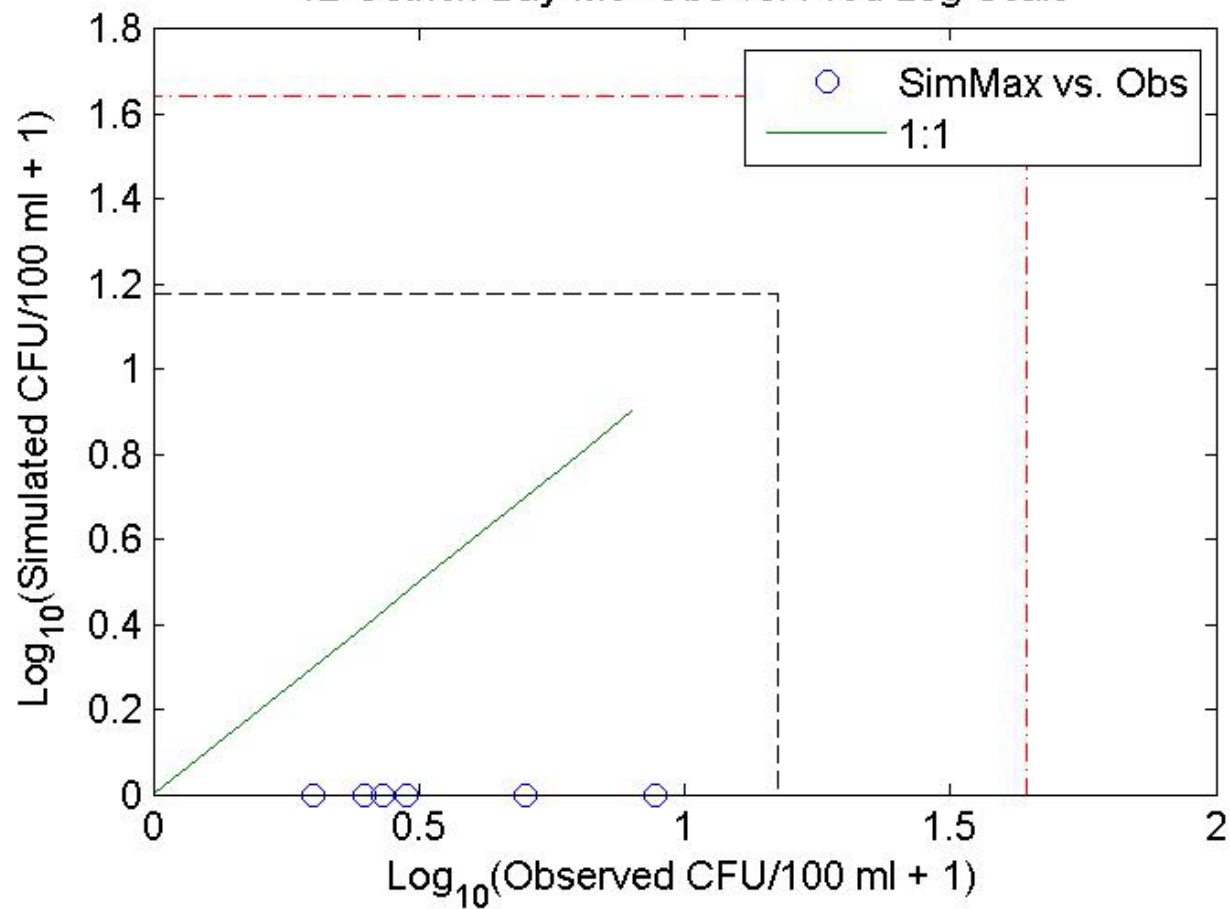
12-Ostrich-Bay-M6- Obs vs. Pred Log Scale
