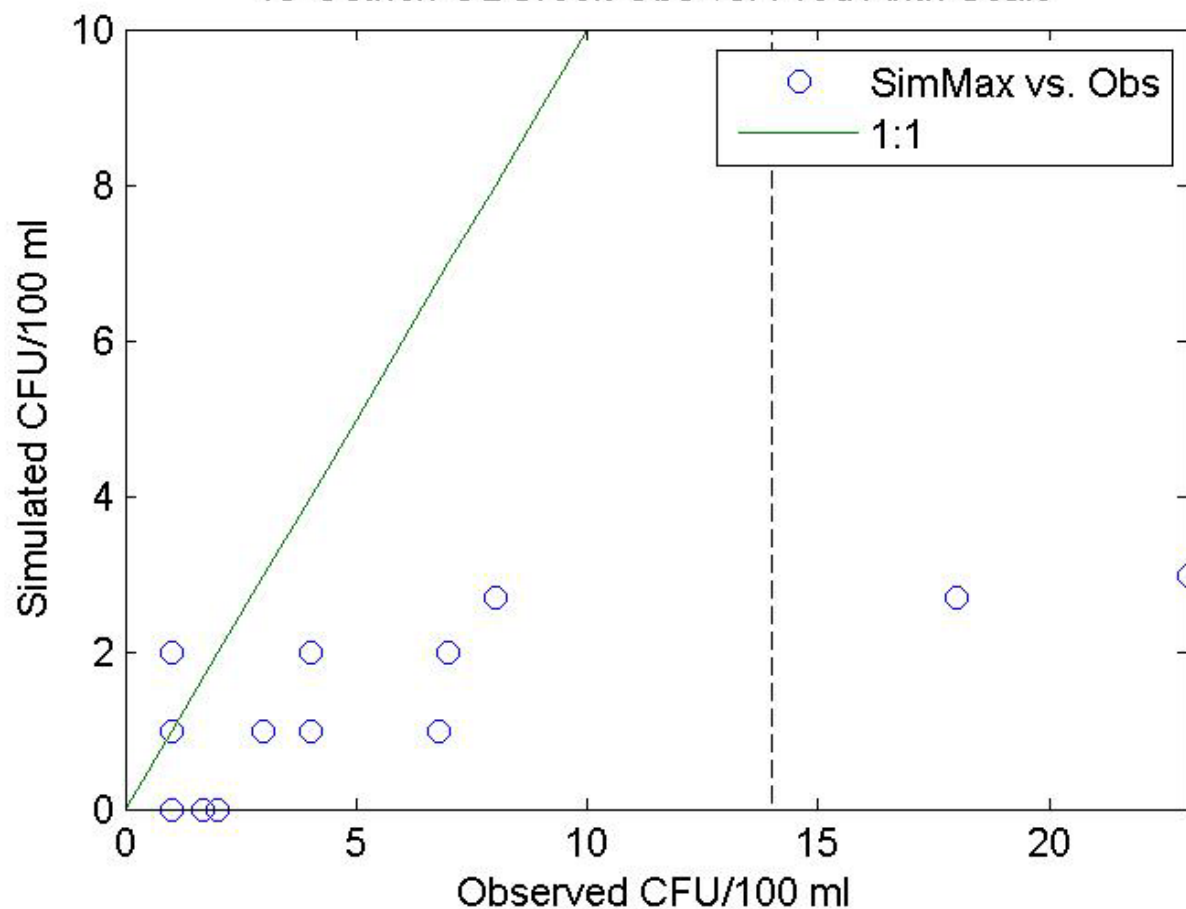
15-Ostrich-OBCreek Obs vs. Pred Arith Scale
