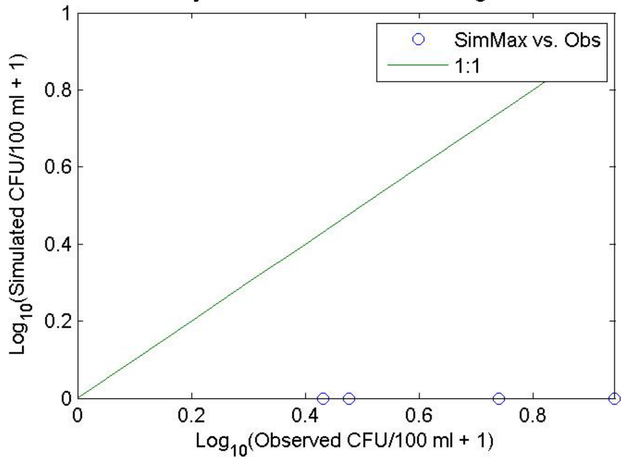
11-Dyes-wShore---- Obs vs. Pred Log Scale
