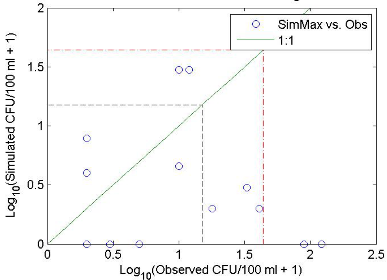
51-SinPO-KarcherCr Obs vs. Pred Log Scale
