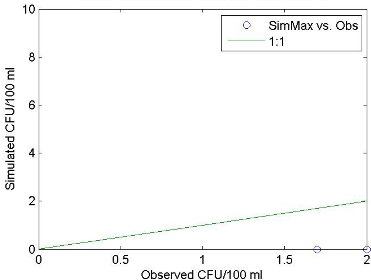
20-POP-IllaheeSPCr Obs vs. Pred Arith Scale
