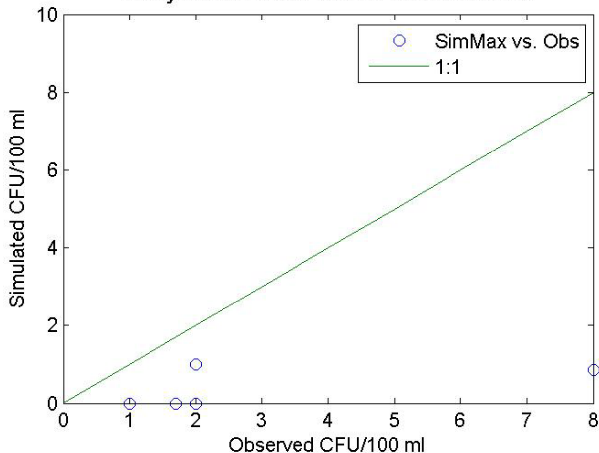
05-Dyes-DY28-Claml Obs vs. Pred Arith Scale
