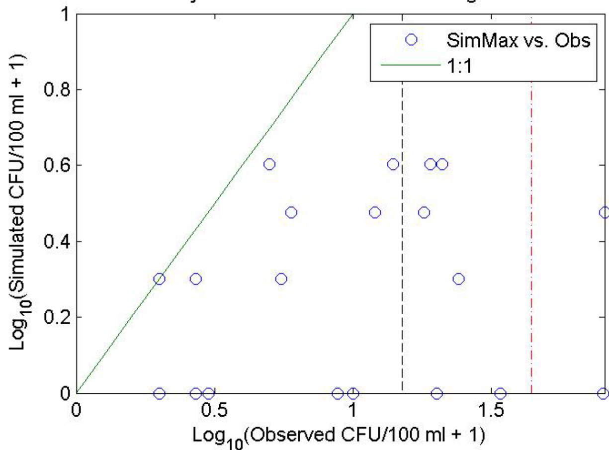
02-Dyes-Chico-Cr-- Obs vs. Pred Log Scale
