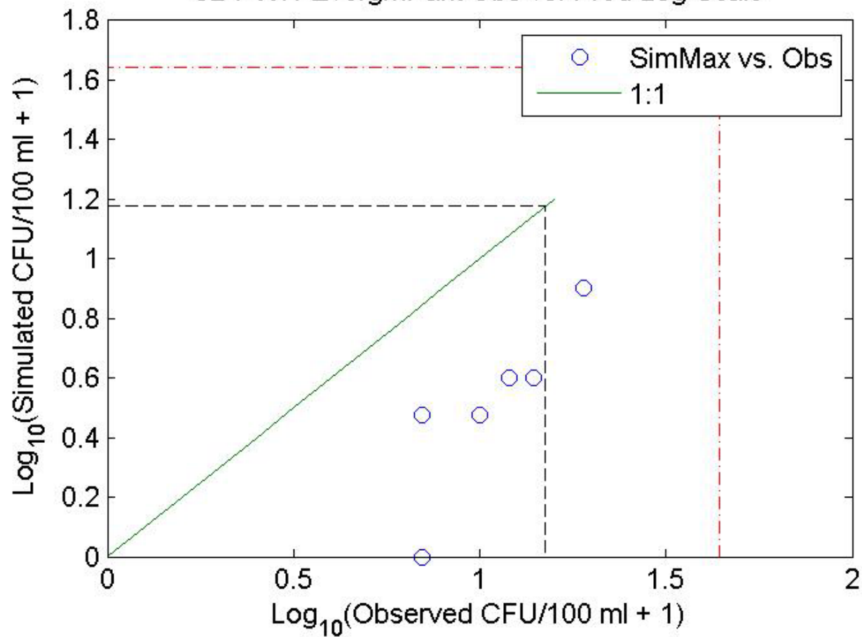
32-PWN-EvergrnPark Obs vs. Pred Log Scale
