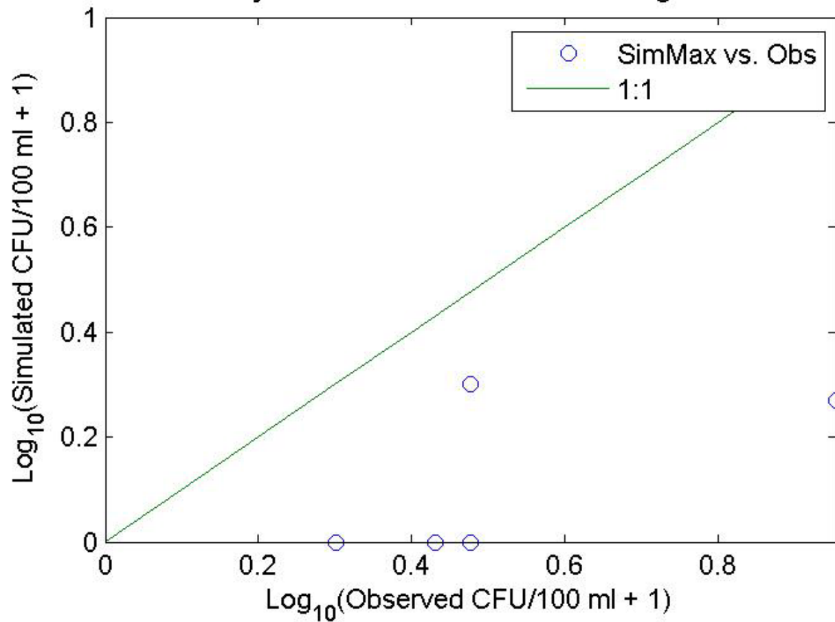
05-Dyes-DY28-Claml Obs vs. Pred Log Scale
