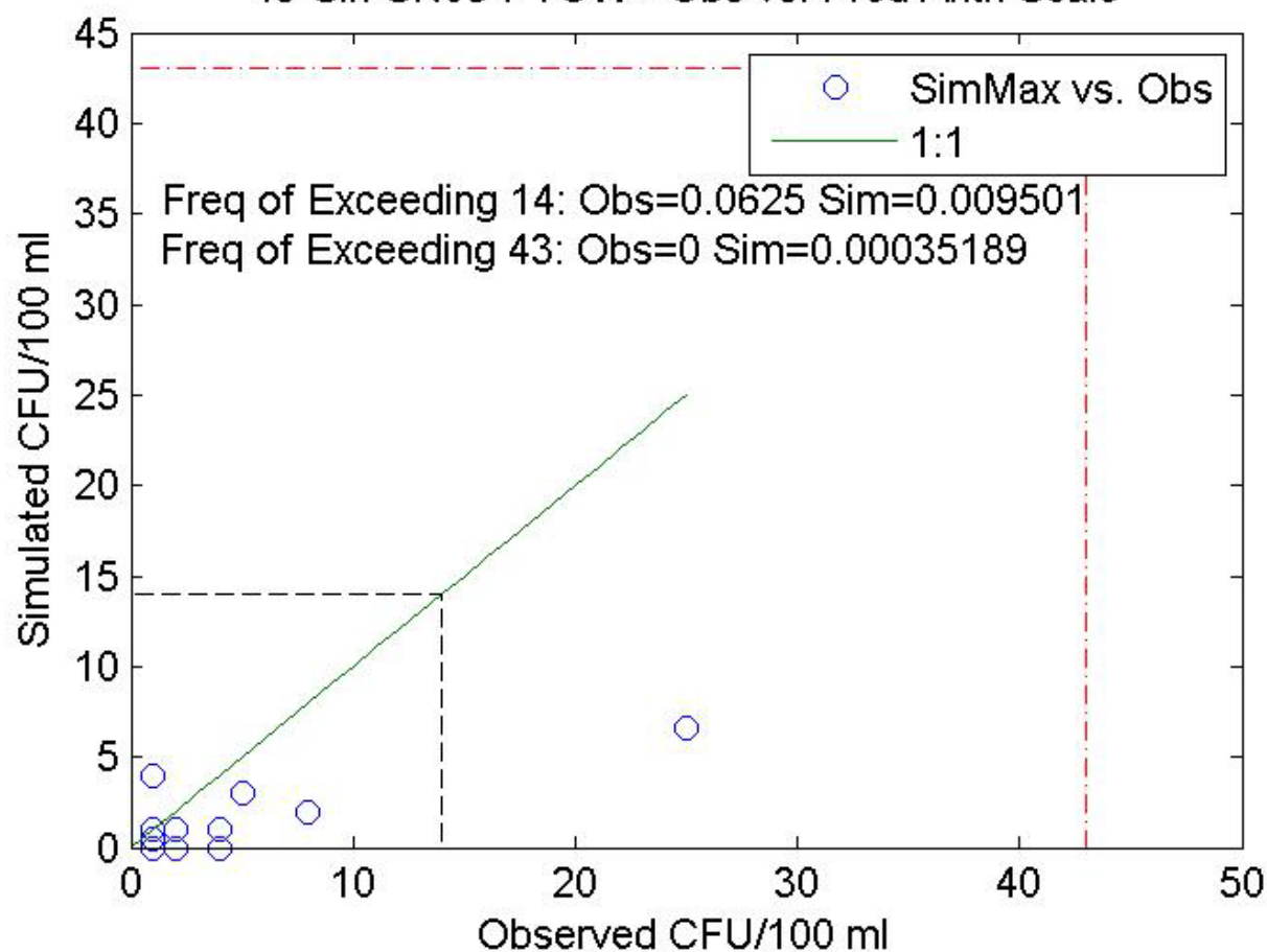
49-Sin-SN03-PTOW-- Obs vs. Pred Arith Scale
