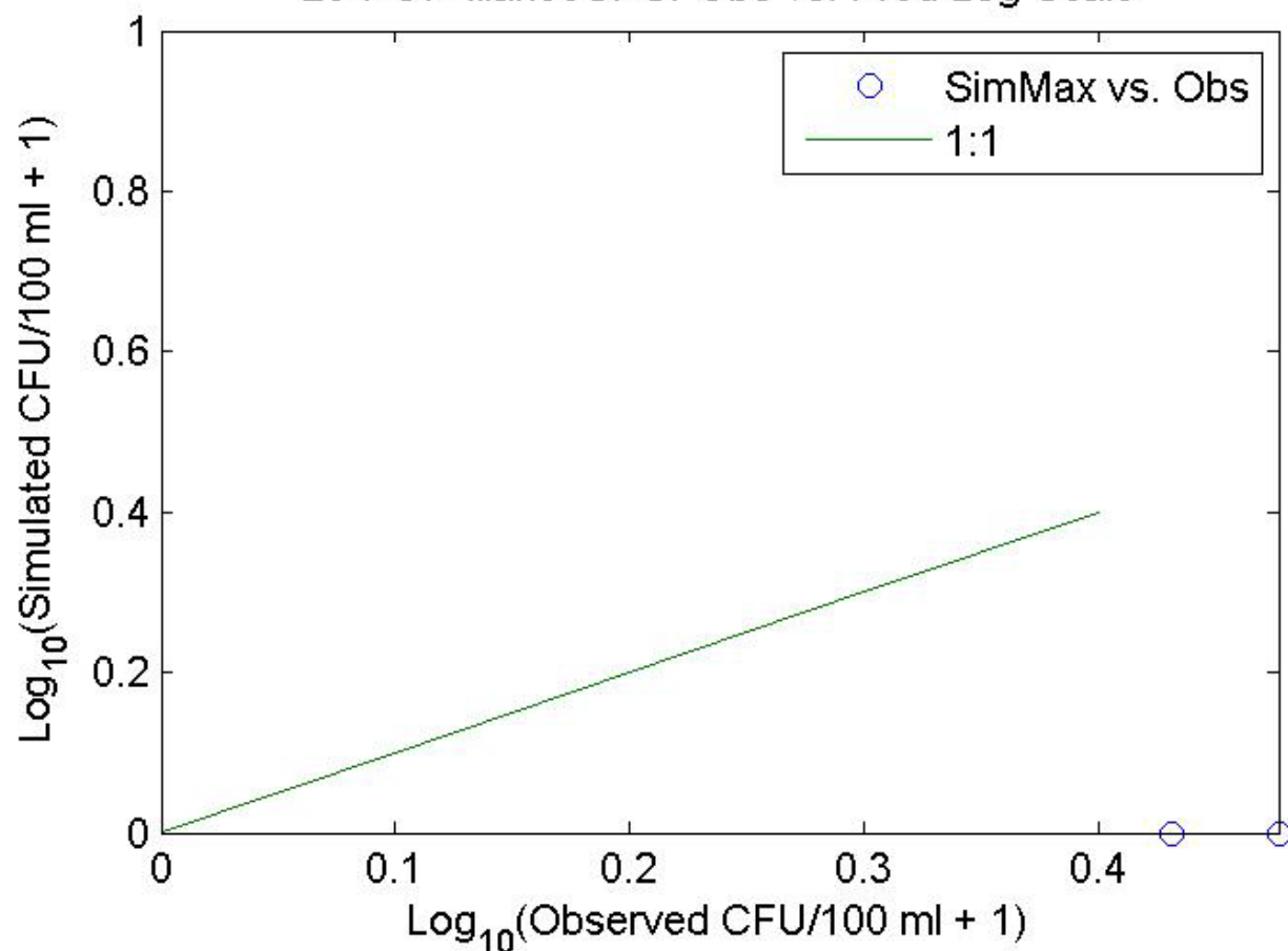
20-POP-IllaheeSPCr Obs vs. Pred Log Scale
