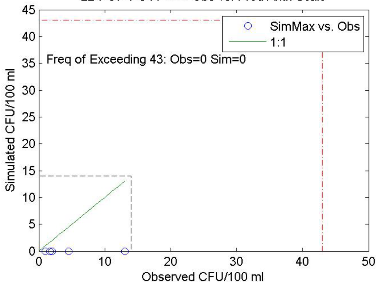
22-POP-PO11----- Obs vs. Pred Arith Scale
