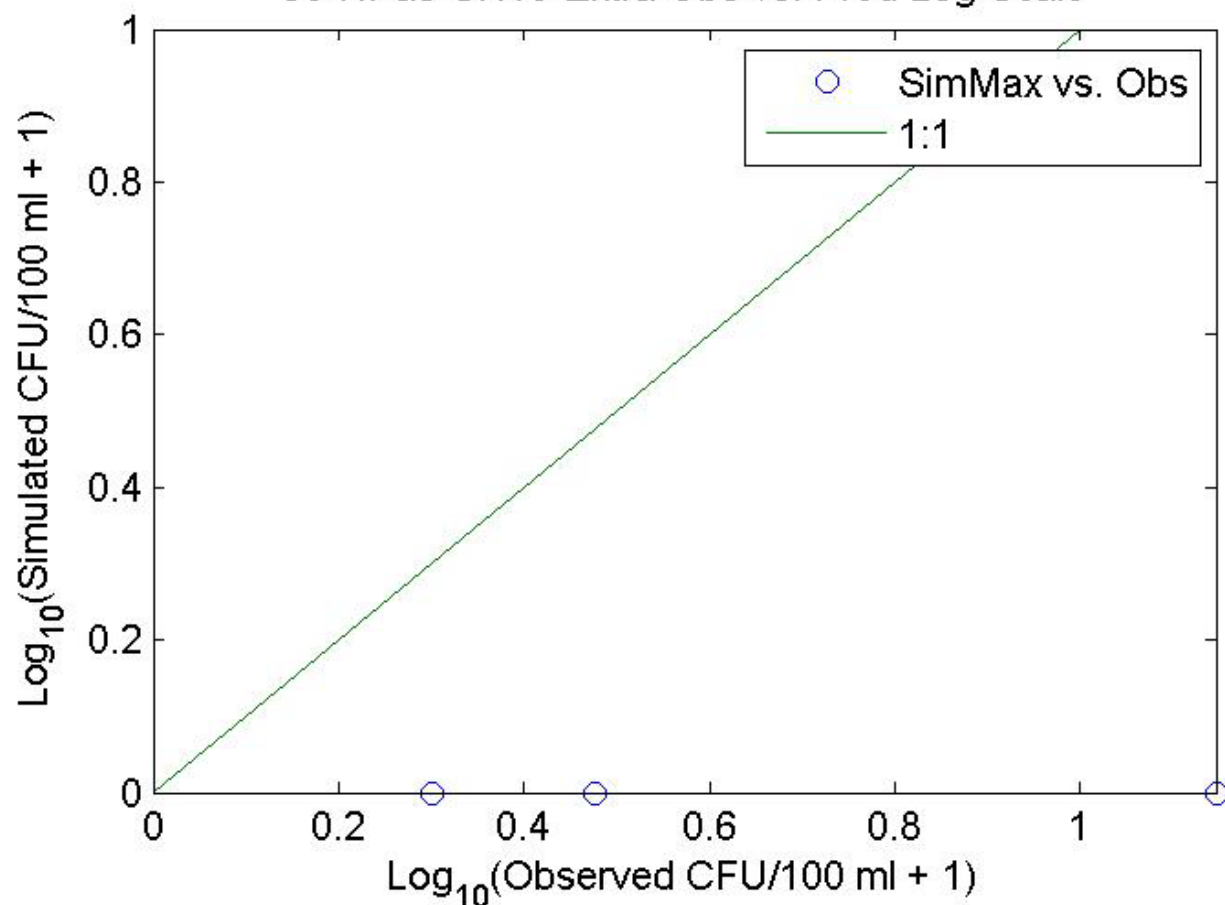
38-RPas-SN18-Entra Obs vs. Pred Log Scale
