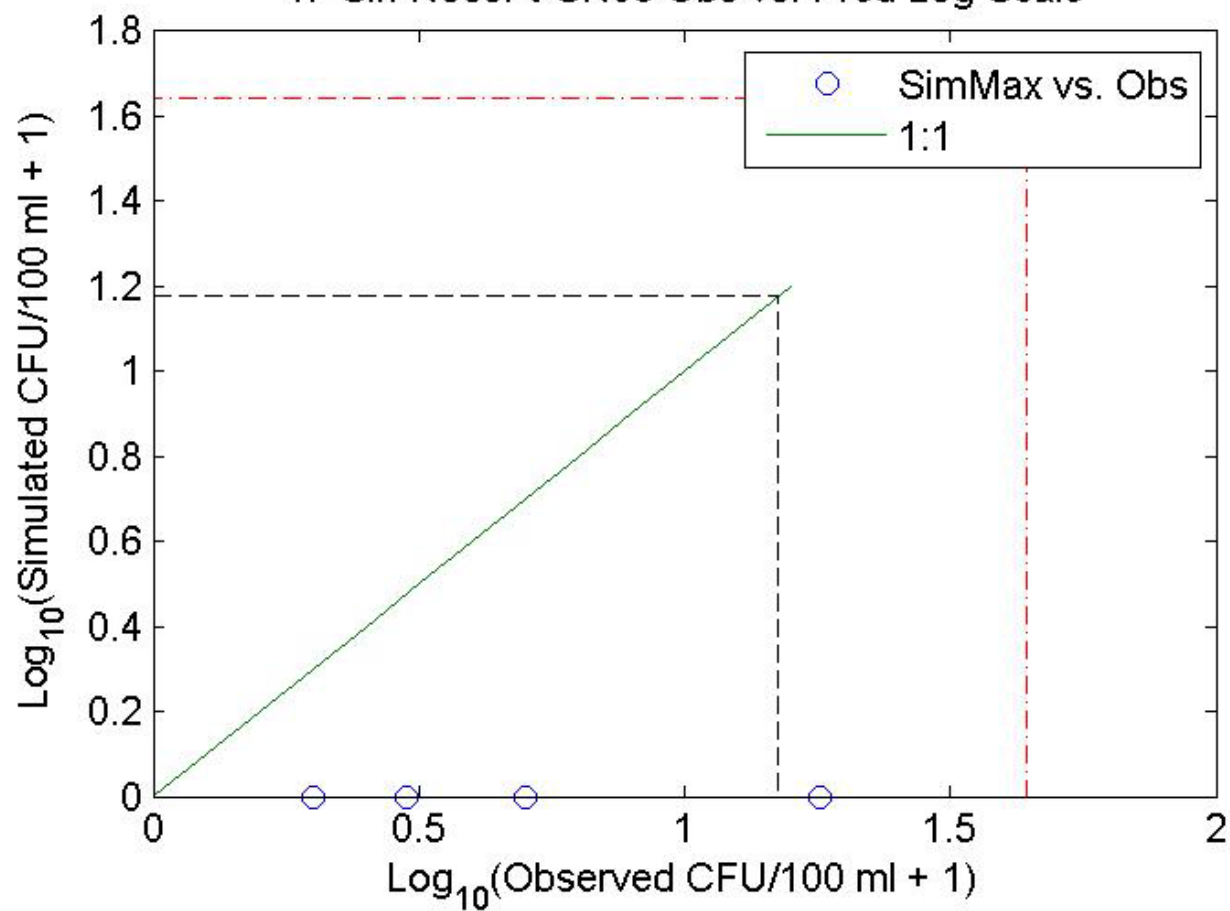
47-Sin-RossPt-SN08 Obs vs. Pred Log Scale
