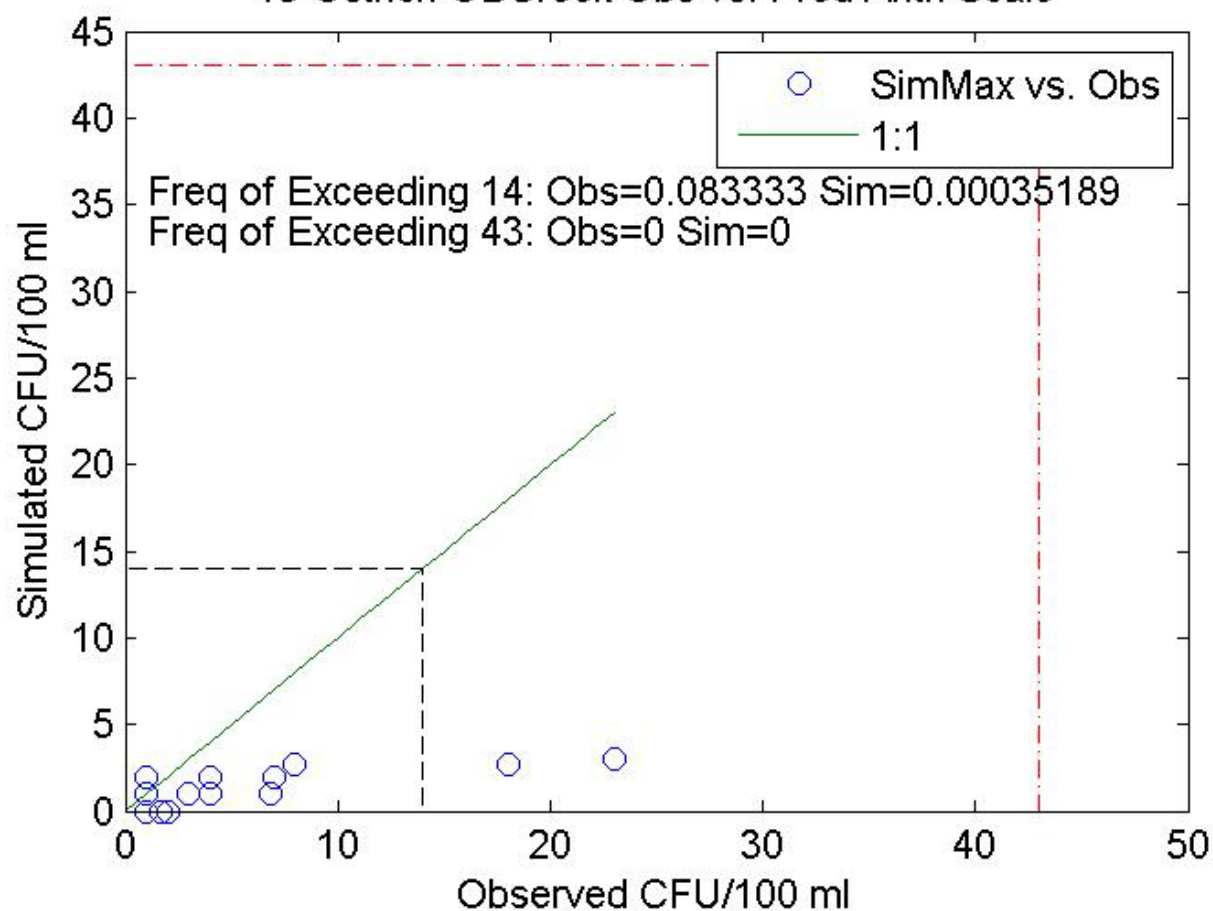
15-Ostrich-OBCreek Obs vs. Pred Arith Scale
