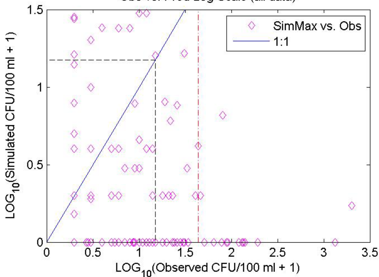
Obs vs. Pred Log Scale (all data)
