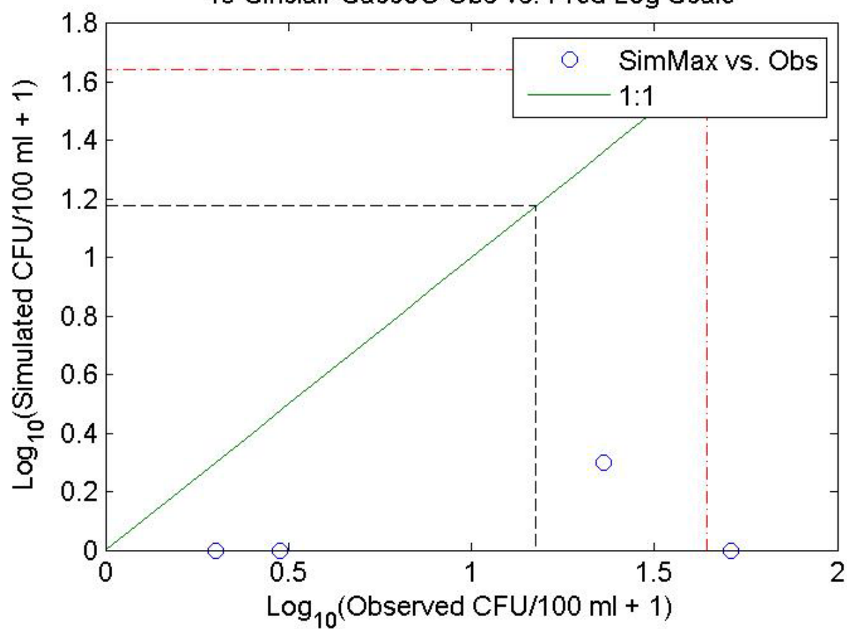
48-Sinclair-SaccoC Obs vs. Pred Log Scale
